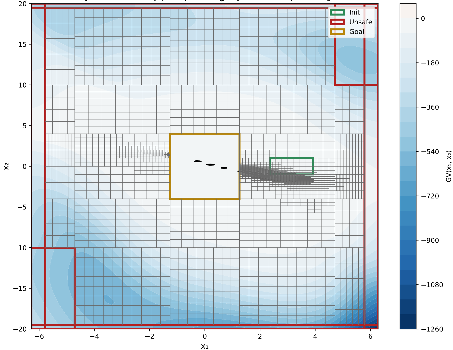
X 1 VS X 2 Epoch 5000 - GV(x) Output Range: [-1257.7720, 0.0806]
