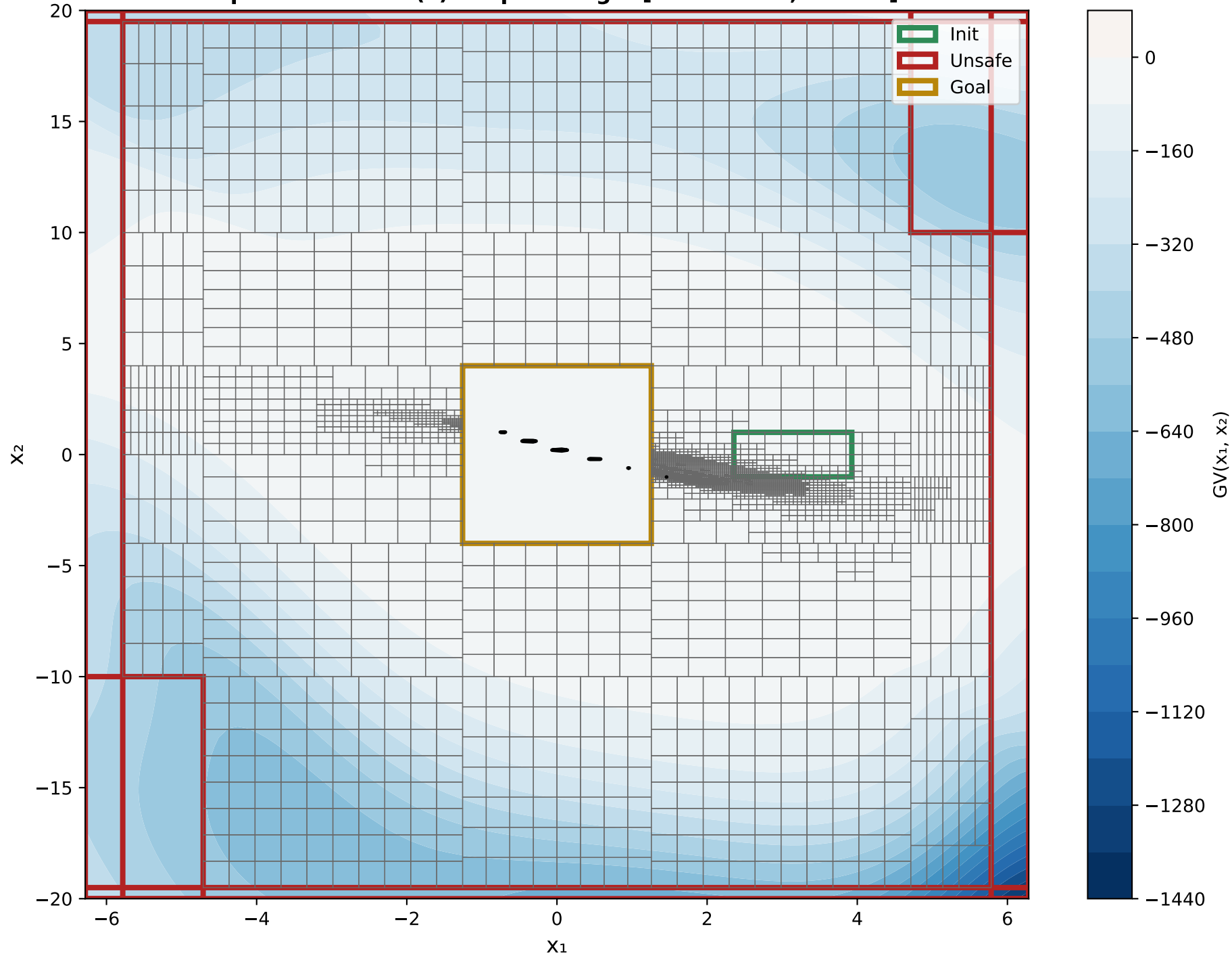
X 1 VS X 2 Epoch 6000 - GV(x) Output Range: [-1401.7236, 0.0450]
