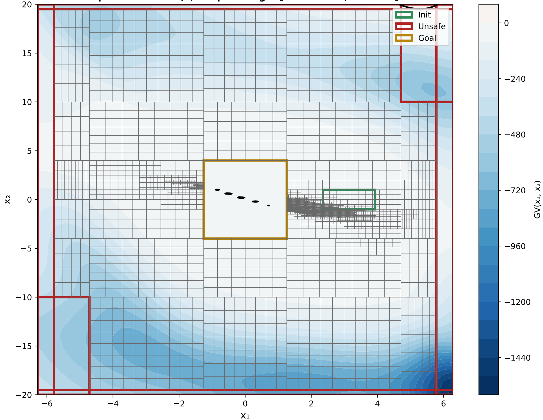
X 1 VS X 2 Epoch 8000 - GV(x) Output Range: [-1543.2844, 31.5234]
