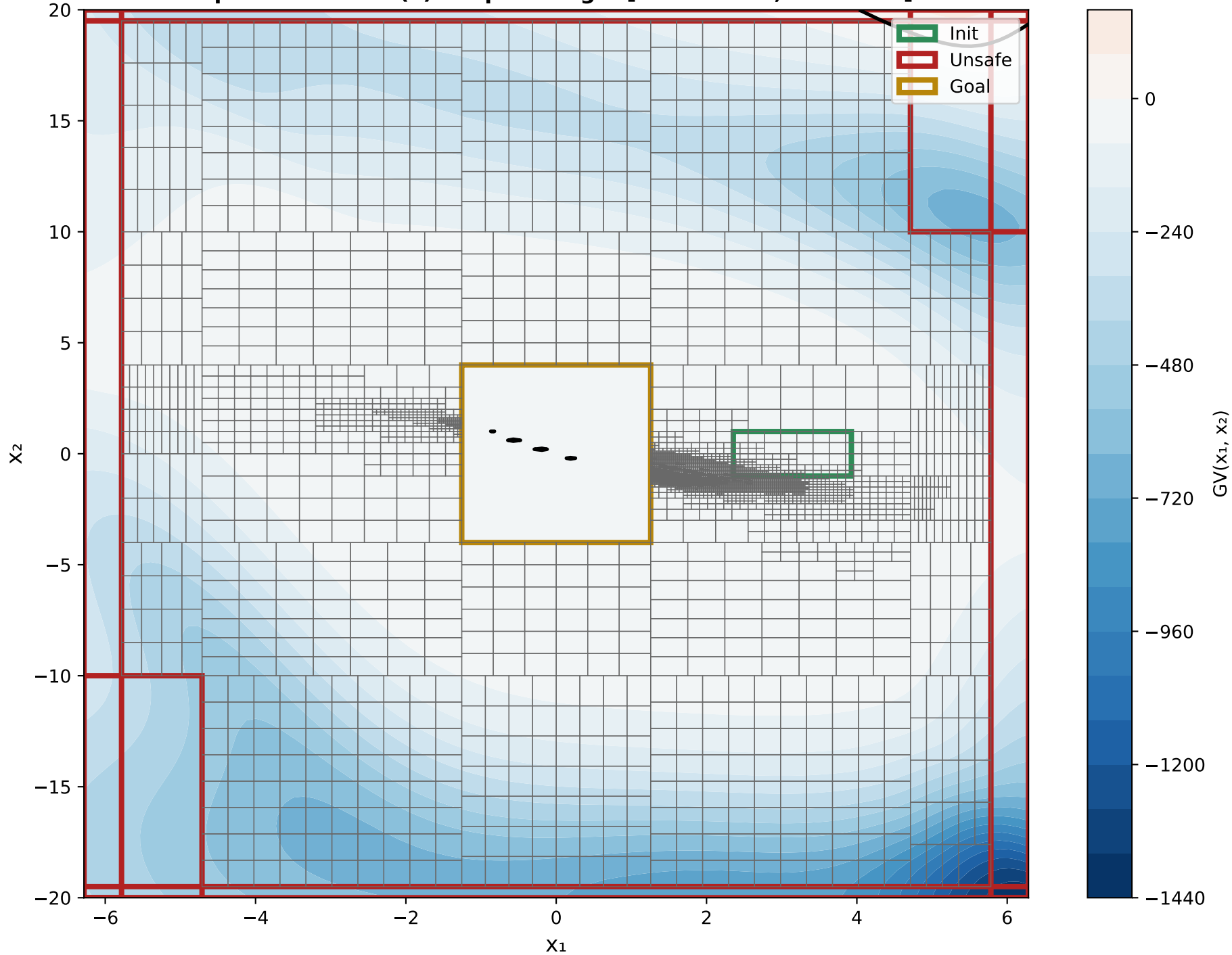
X 1 VS X 2 Epoch 9000 - GV(x) Output Range: [-1425.1548, 102.0612]
