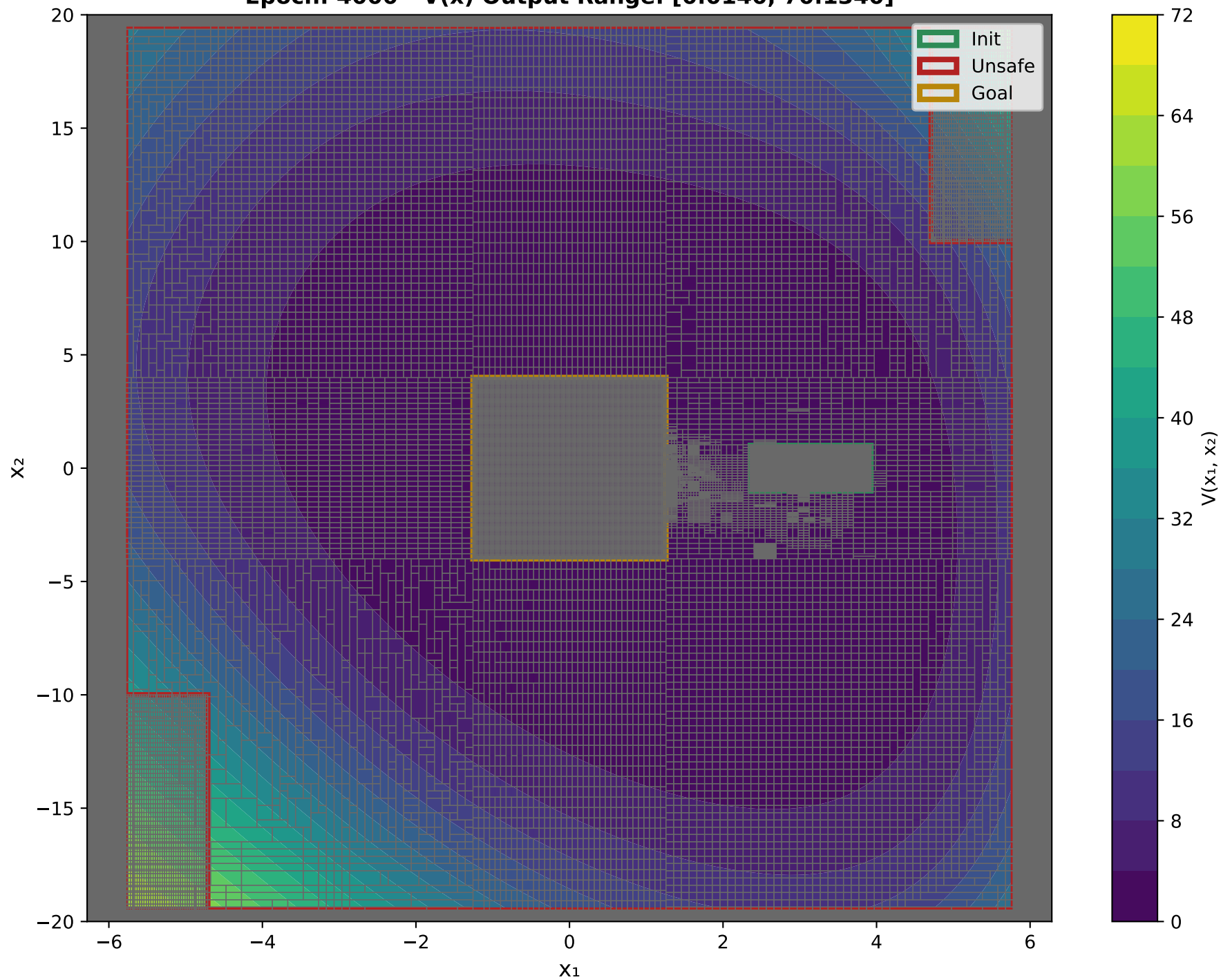
X 1 VS X 2 Epoch: 4000 - V(x) Output Range: [0.0140, 70.1340]
