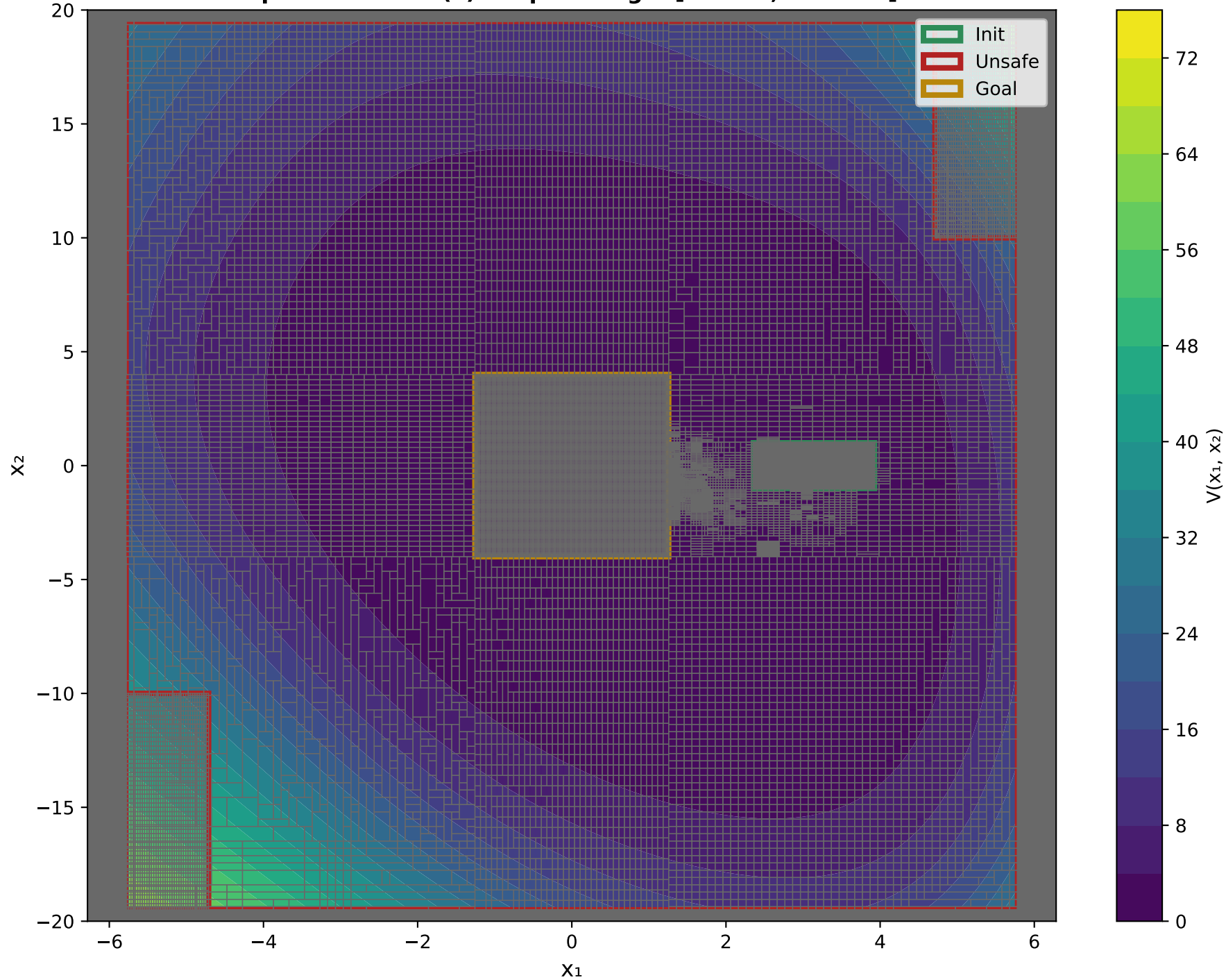
X 1 VS X 2 Epoch: 5000 - V(x) Output Range: [0.0363, 74.8411]
