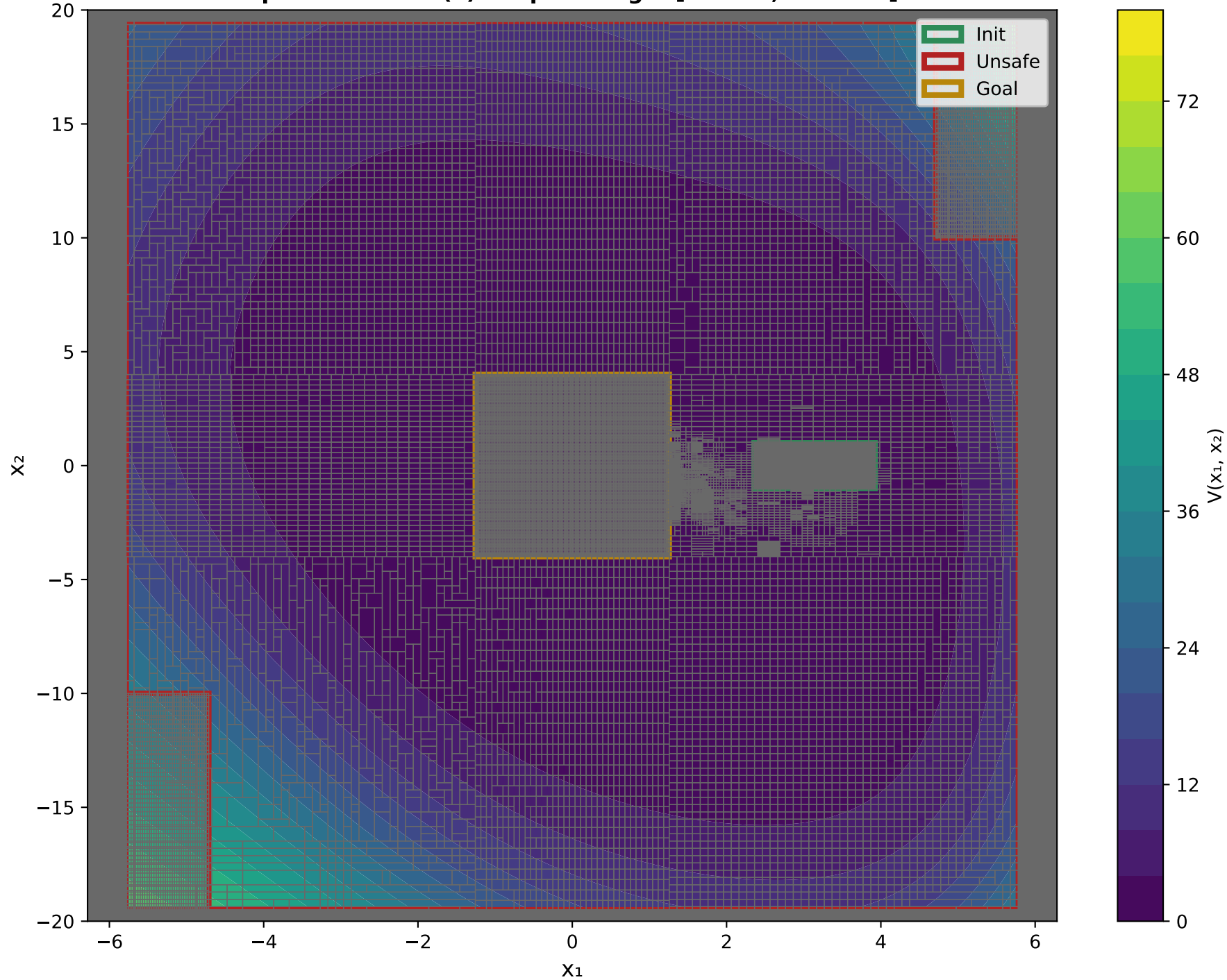
X 1 VS X 2 Epoch: 6000 - V(x) Output Range: [0.0750, 76.3455]
