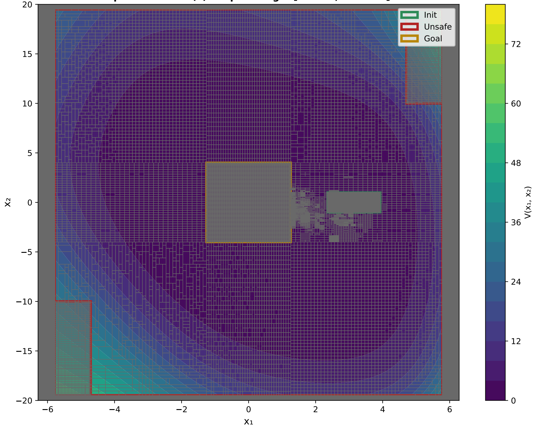
X 1 VS X 2 Epoch: 7000 - V(x) Output Range: [0.0876, 79.4879]
