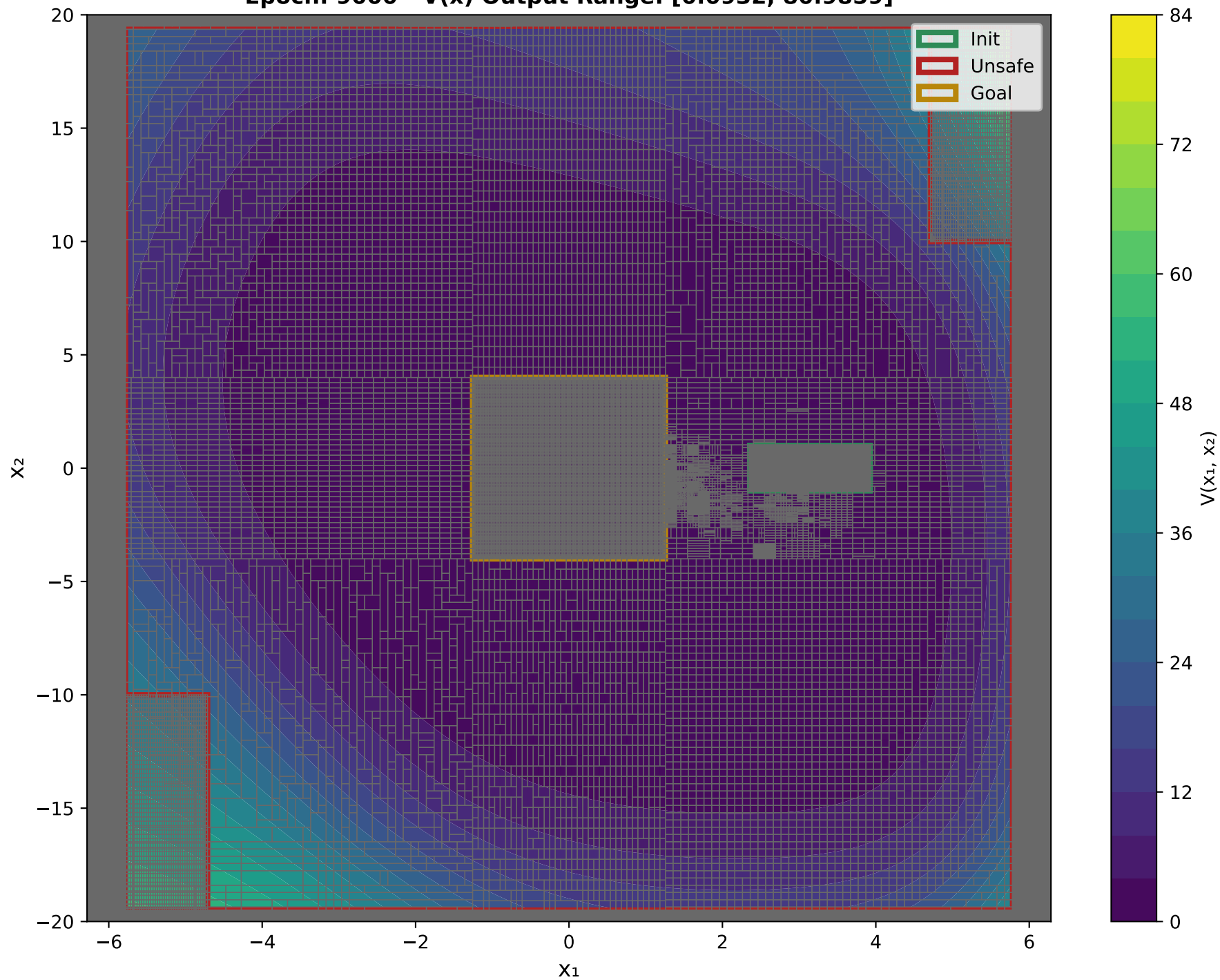
X 1 VS X 2 Epoch: 9000 - V(x) Output Range: [0.0932, 80.9859]
