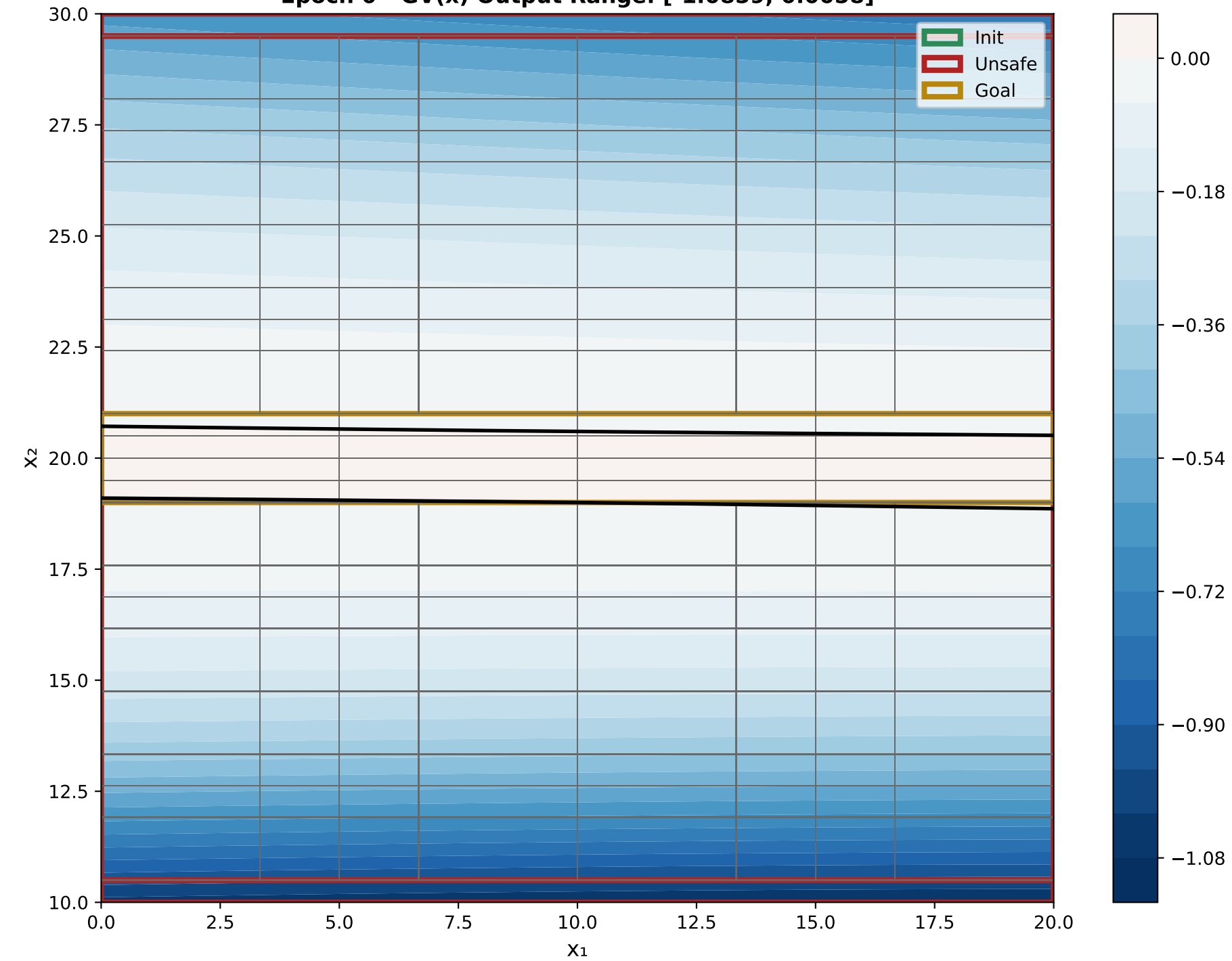
X 1 VS X 2 Epoch 0 - GV(x) Output Range: [-1.0859, 0.0058]
