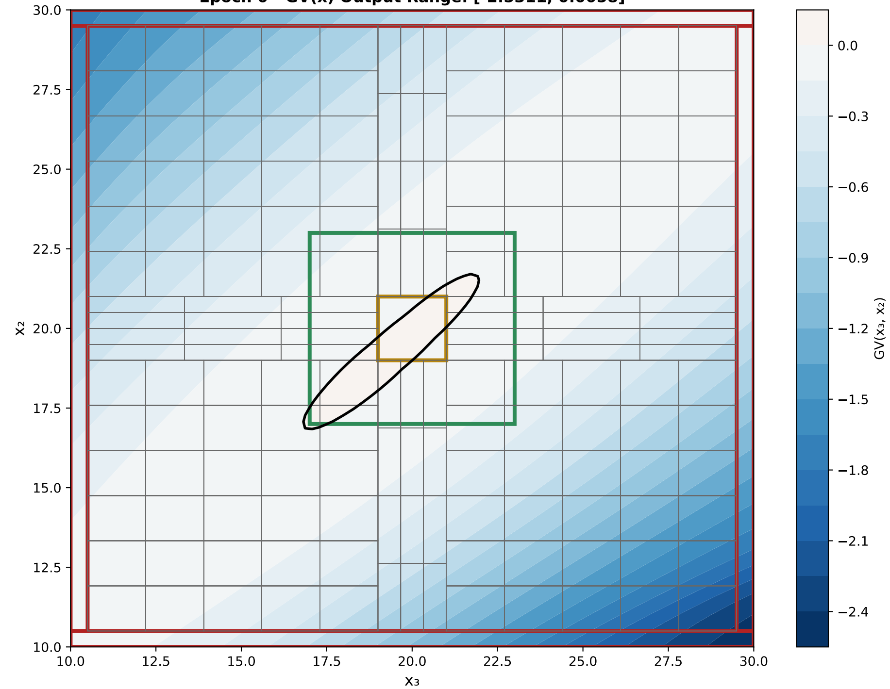
X 3 VS X 2 Epoch 0 - GV(x) Output Range: [-2.5311, 0.0058]
