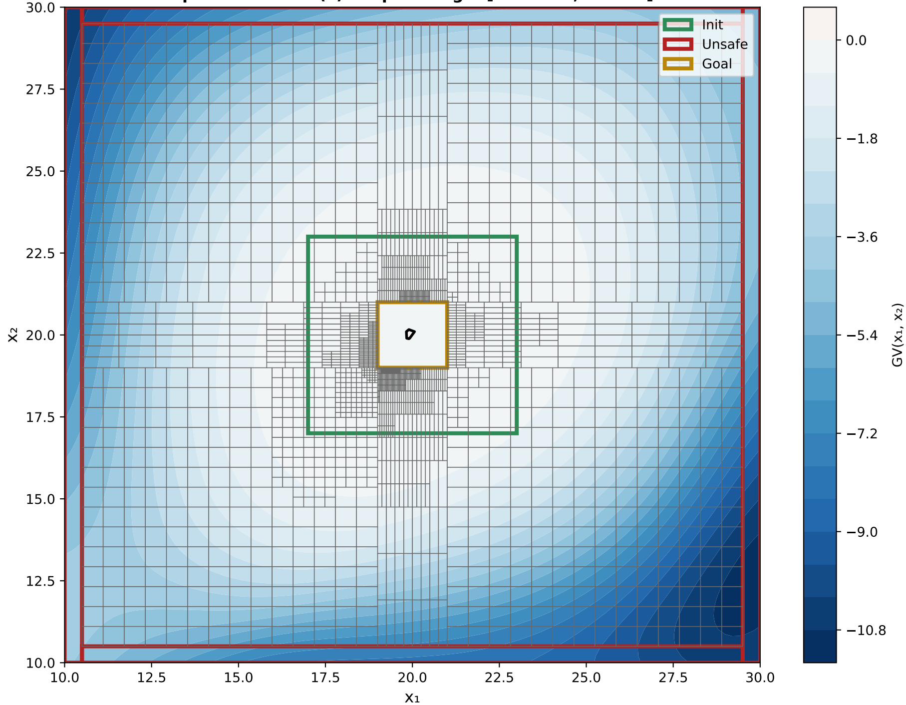
X 1 VS X 2 Epoch 2000 - GV(x) Output Range: [-11.1036, 0.0002]
