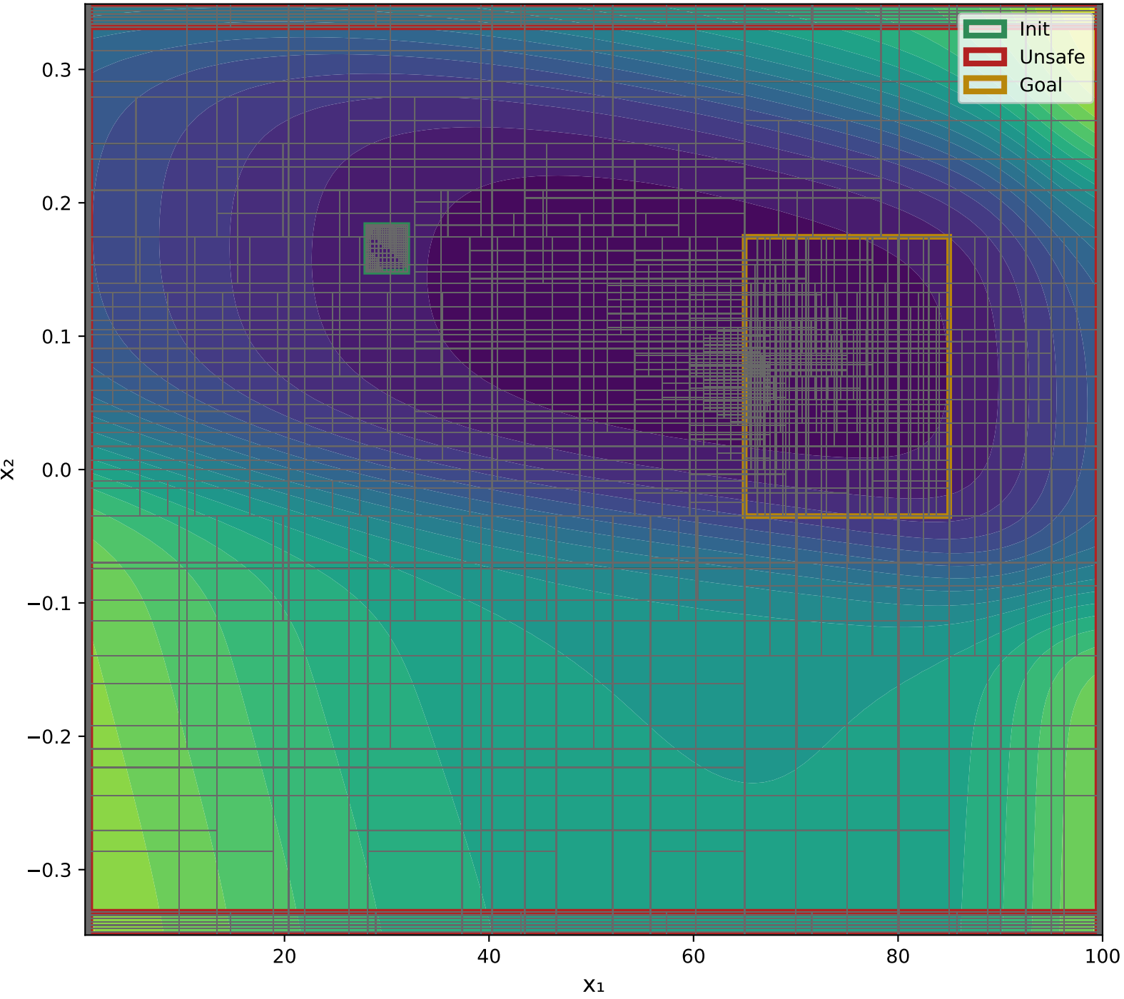
X 1 VS X 2 Epoch: 1000 - V(x) Output Range: [2.4949, 40.7716]
