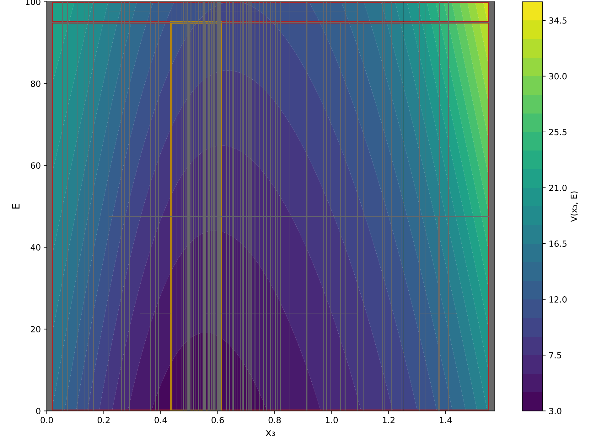
X 3 VS E Epoch: 1000 - V(x) Output Range: [3.5613, 34.9701]
