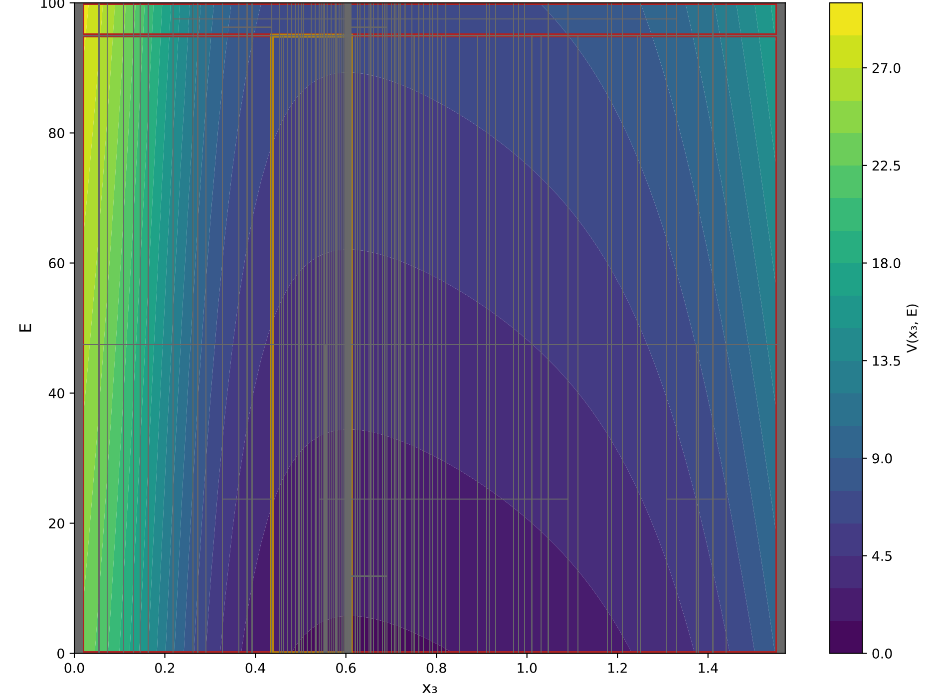
X 3 VS E Epoch: 4000 - V(x) Output Range: [1.2084, 29.7580]
