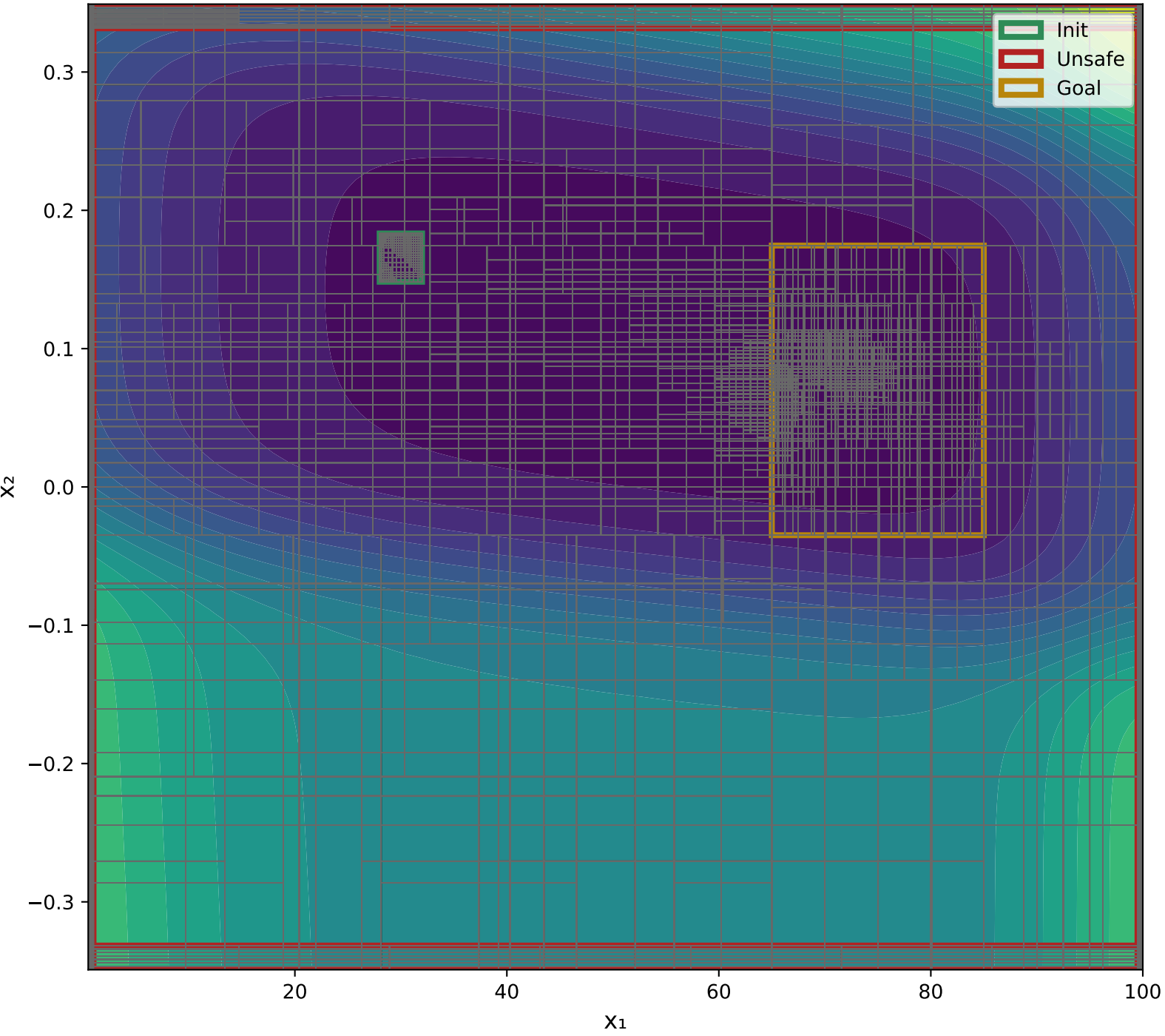
X 1 VS X 2 Epoch: 4000 - V(x) Output Range: [2.9226, 40.4533]
