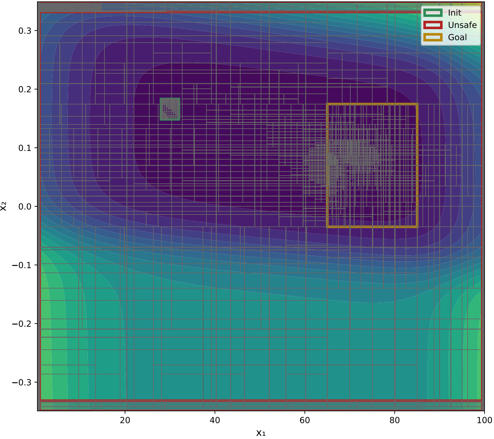
X 1 VS X 2 Epoch: 5000 - V(x) Output Range: [2.9135, 39.4195]
