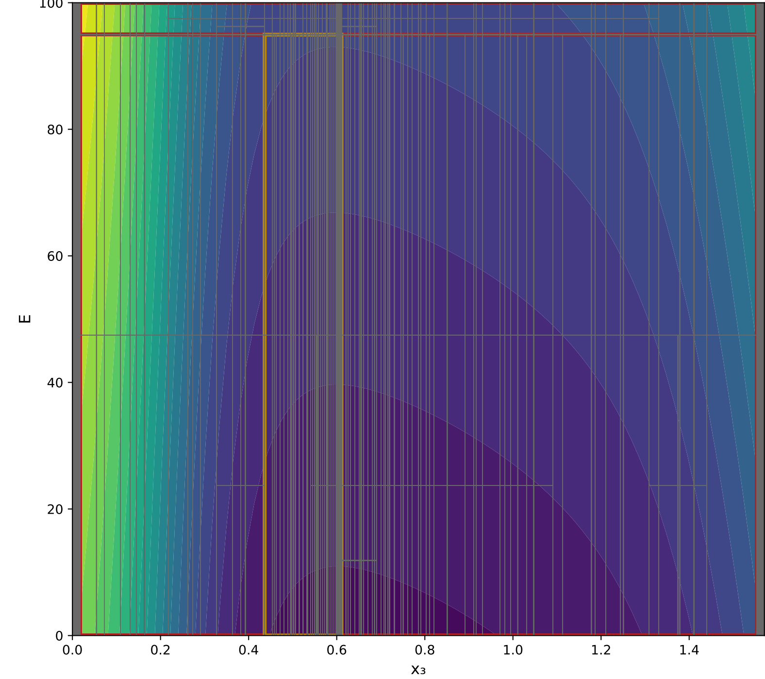
X 3 VS E Epoch: 5000 - V(x) Output Range: [0.9555, 31.2968]
