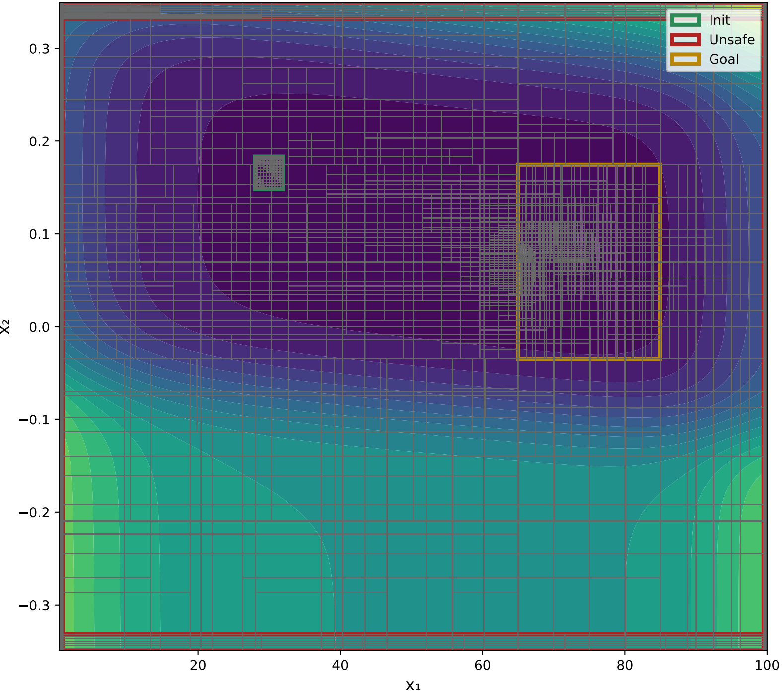
X 1 VS X 2 Epoch: 7000 - V(x) Output Range: [2.8421, 38.8825]
