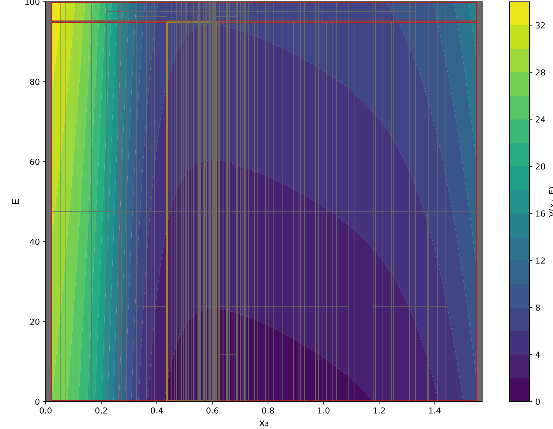
X 3 VS E Epoch: 7000 - V(x) Output Range: [0.8689, 33.9067]
