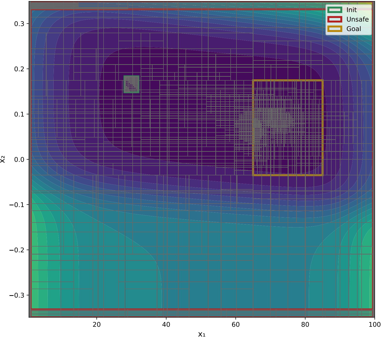
X 1 VS X 2 Epoch: 8000 - V(x) Output Range: [2.8671, 40.2954]
