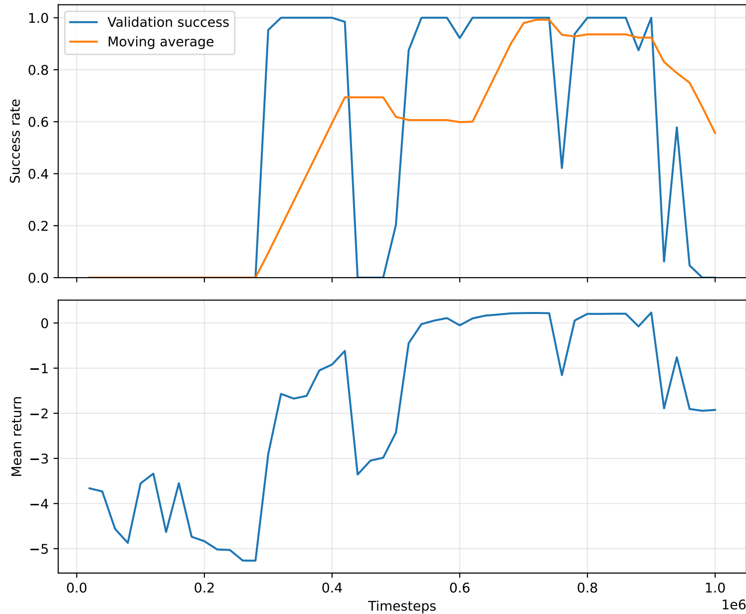
XV-15 SB3 PPO teacher training
