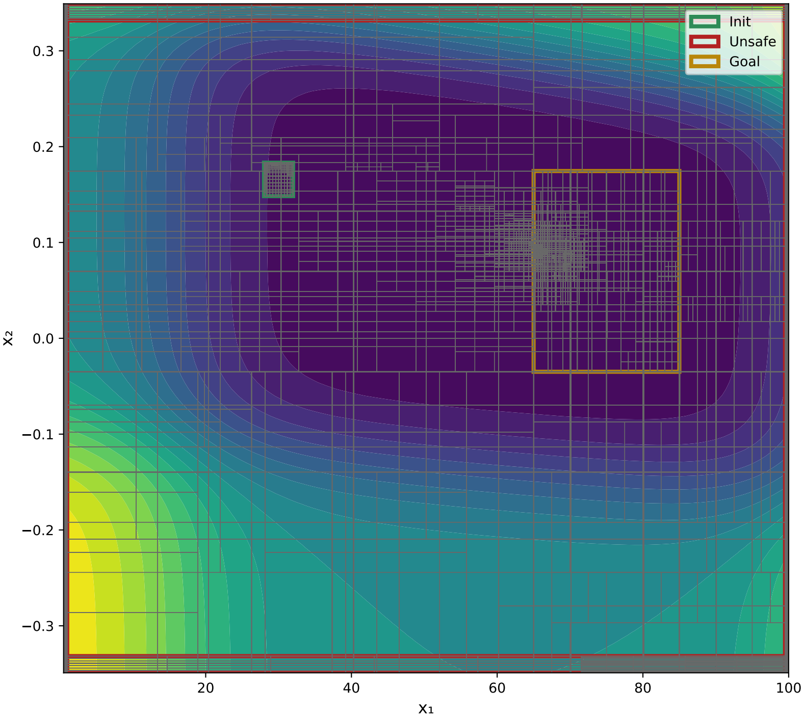
X 1 VS X 2 Epoch: 3000 - V(x) Output Range: [0.0291, 71.1411]
