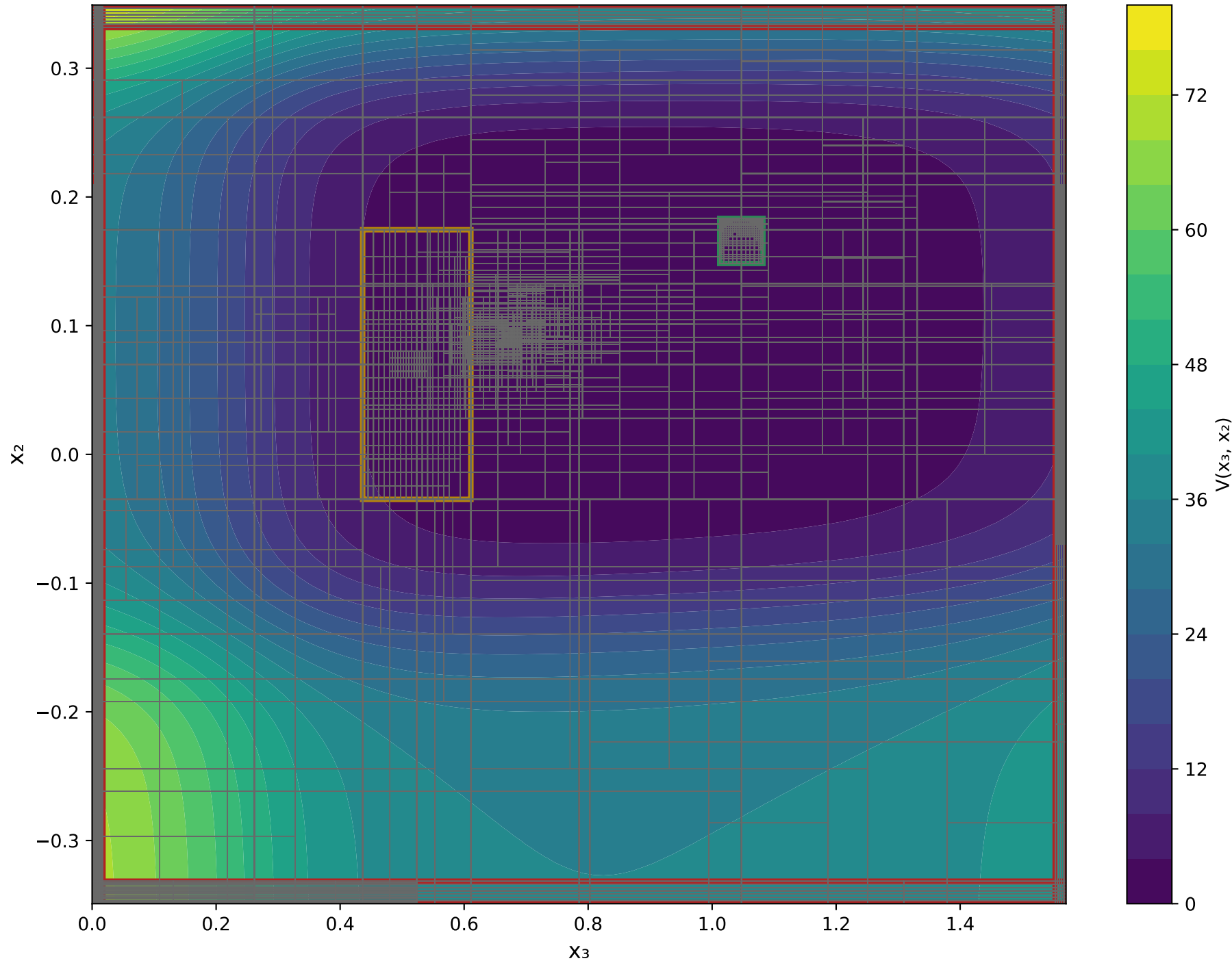
X 3 VS X 2 Epoch: 3000 - V(x) Output Range: [0.1014, 77.3205]
