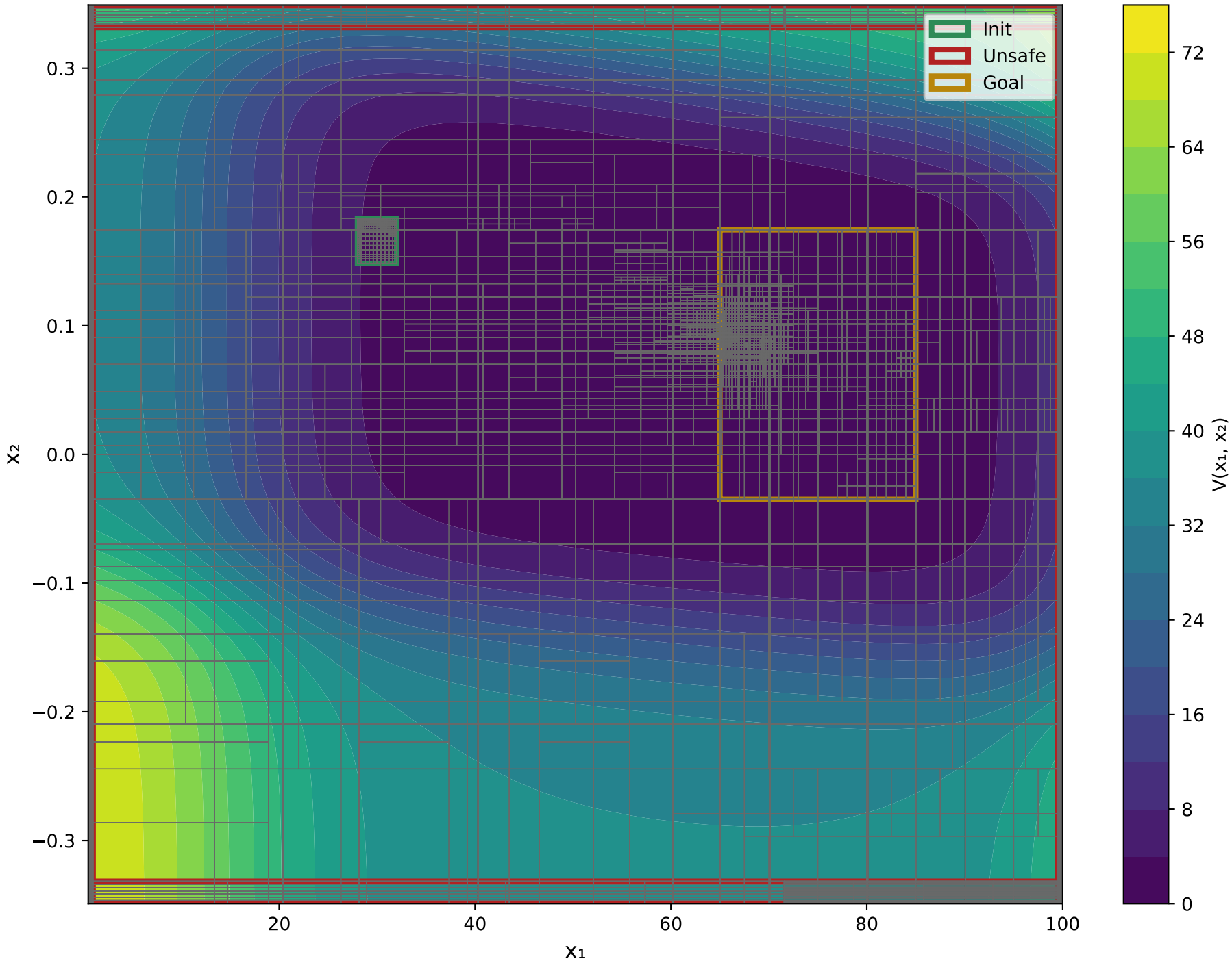
X 1 VS X 2 Epoch: 4000 - V(x) Output Range: [0.0377, 72.4394]
