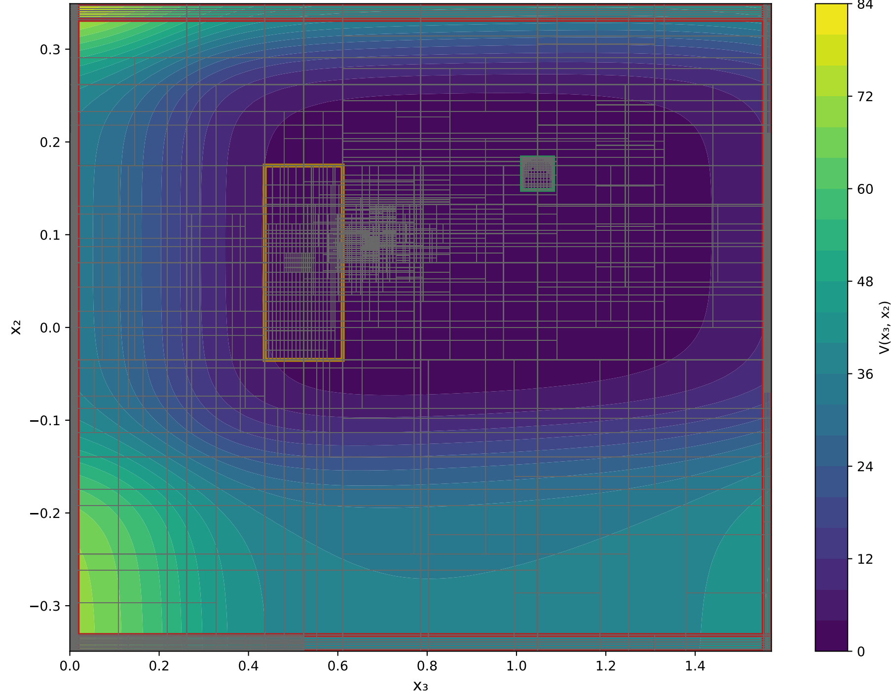
X 3 VS X 2 Epoch: 4000 - V(x) Output Range: [0.1086, 80.8982]
