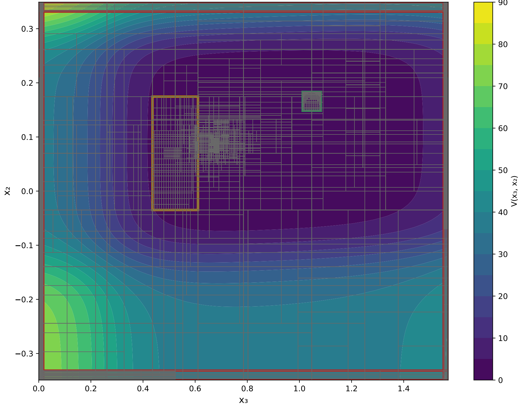
X 3 VS X 2 Epoch: 7000 - V(x) Output Range: [0.1712, 86.3615]
