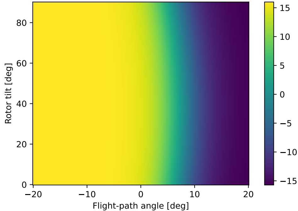
Learned control — Airspeed [m/s] = 75 Angle of attack [deg]
