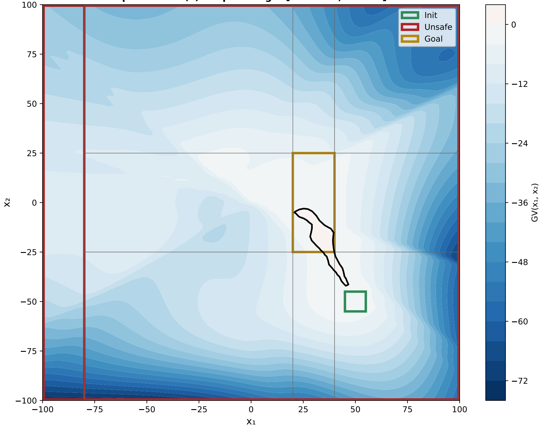
X 1 VS X 2 Epoch 0 - GV(x) Output Range: [-74.7271, 0.4193]
