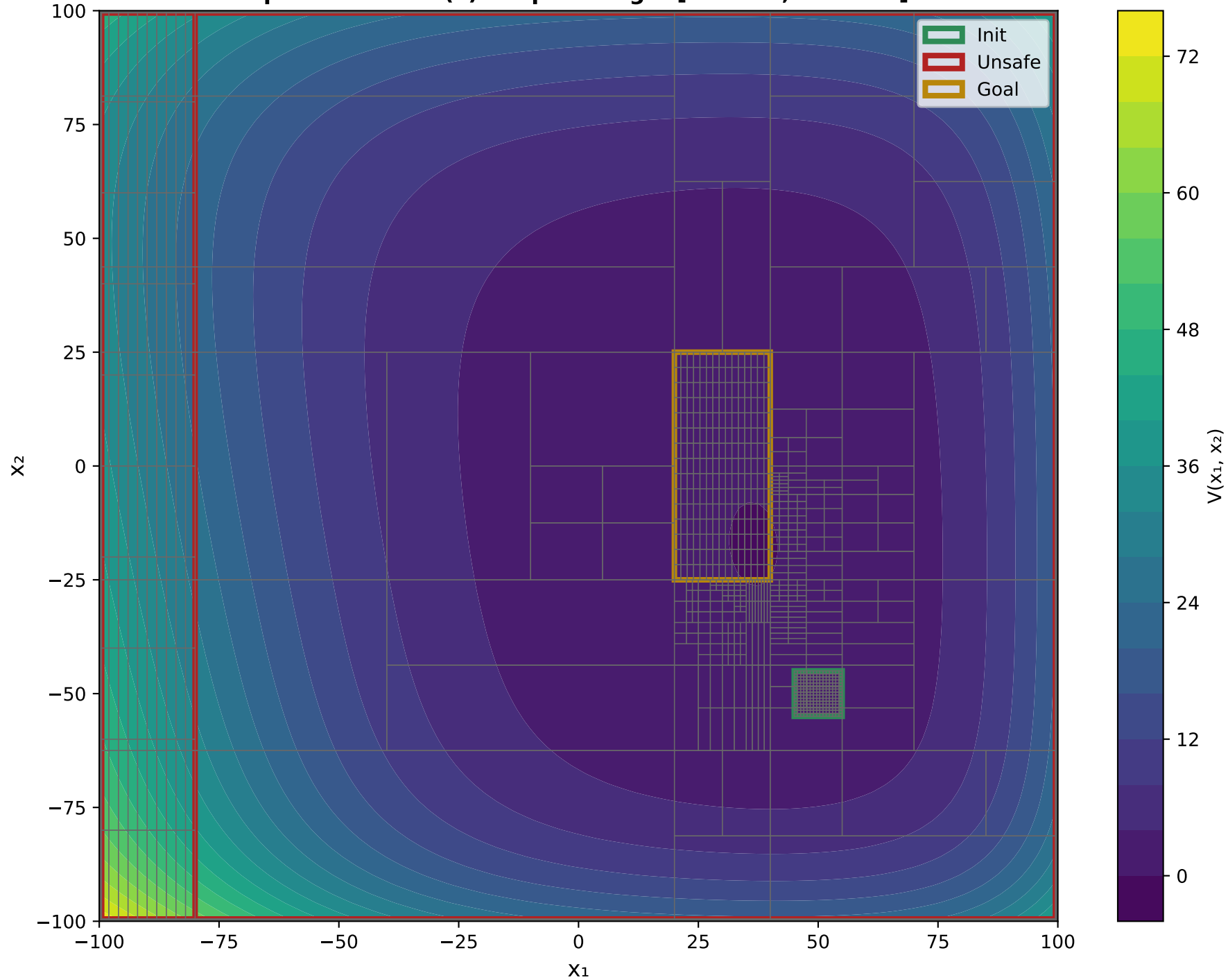
x_1 VS x_2 Epoch: 2000 - V(x) Output Range: [-0.0285, 75.8211]
