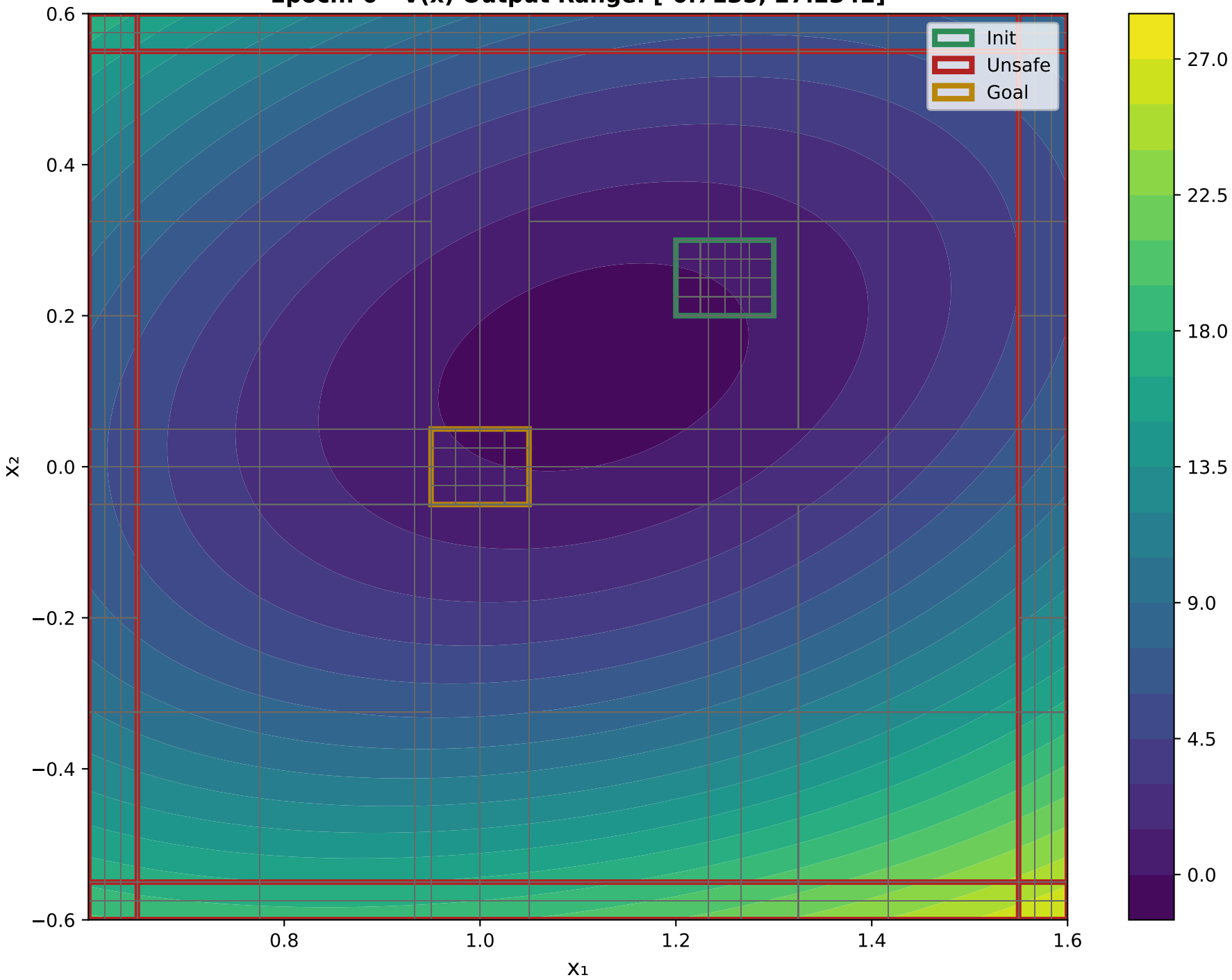
X 1 VS X 2 Epoch: 0 - V(x) Output Range: [-0.7135, 27.2342]
