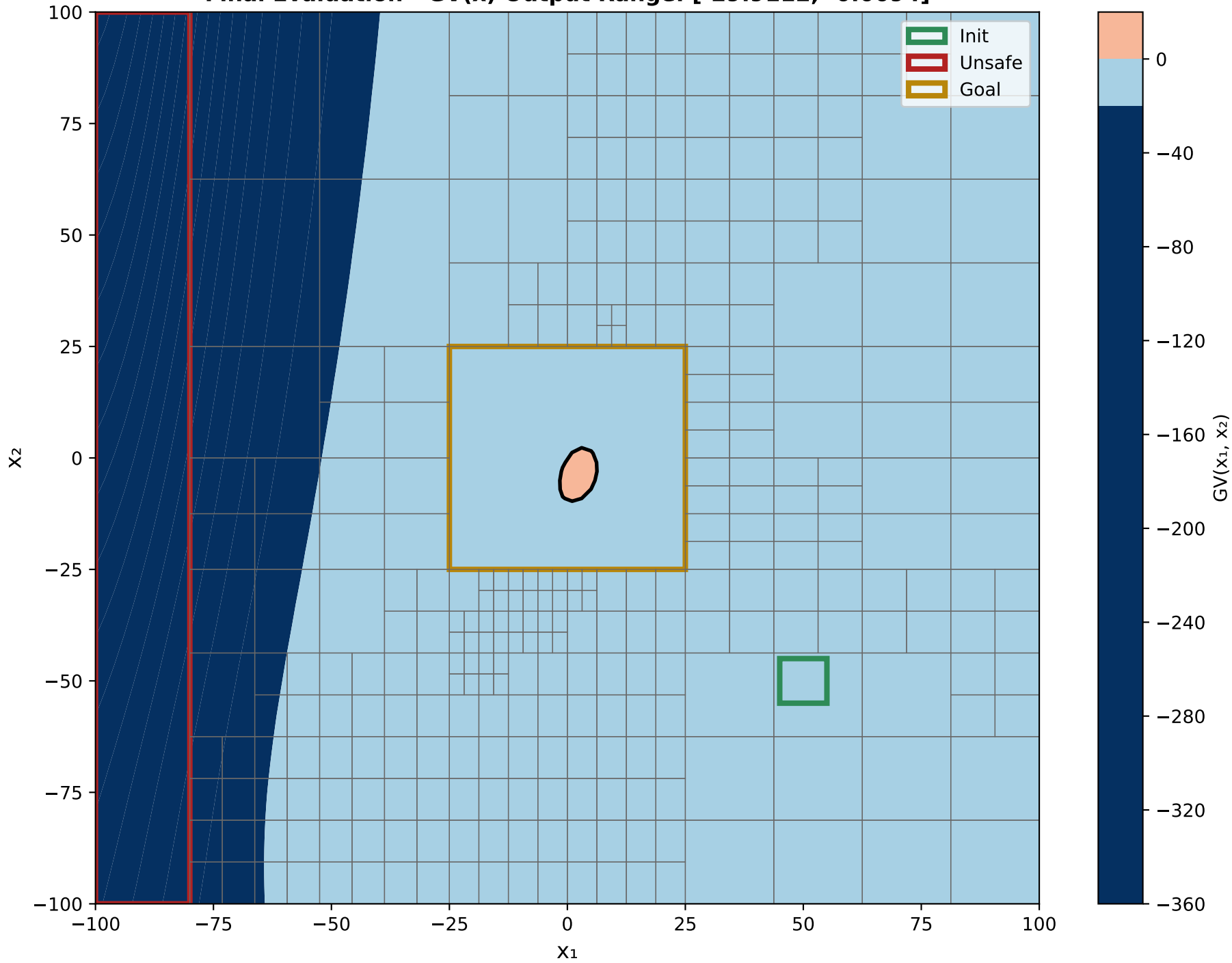
X 1 VS X 2 Final Evaluation - GV(x) Output Range: [-29.9112, -0.0094]
