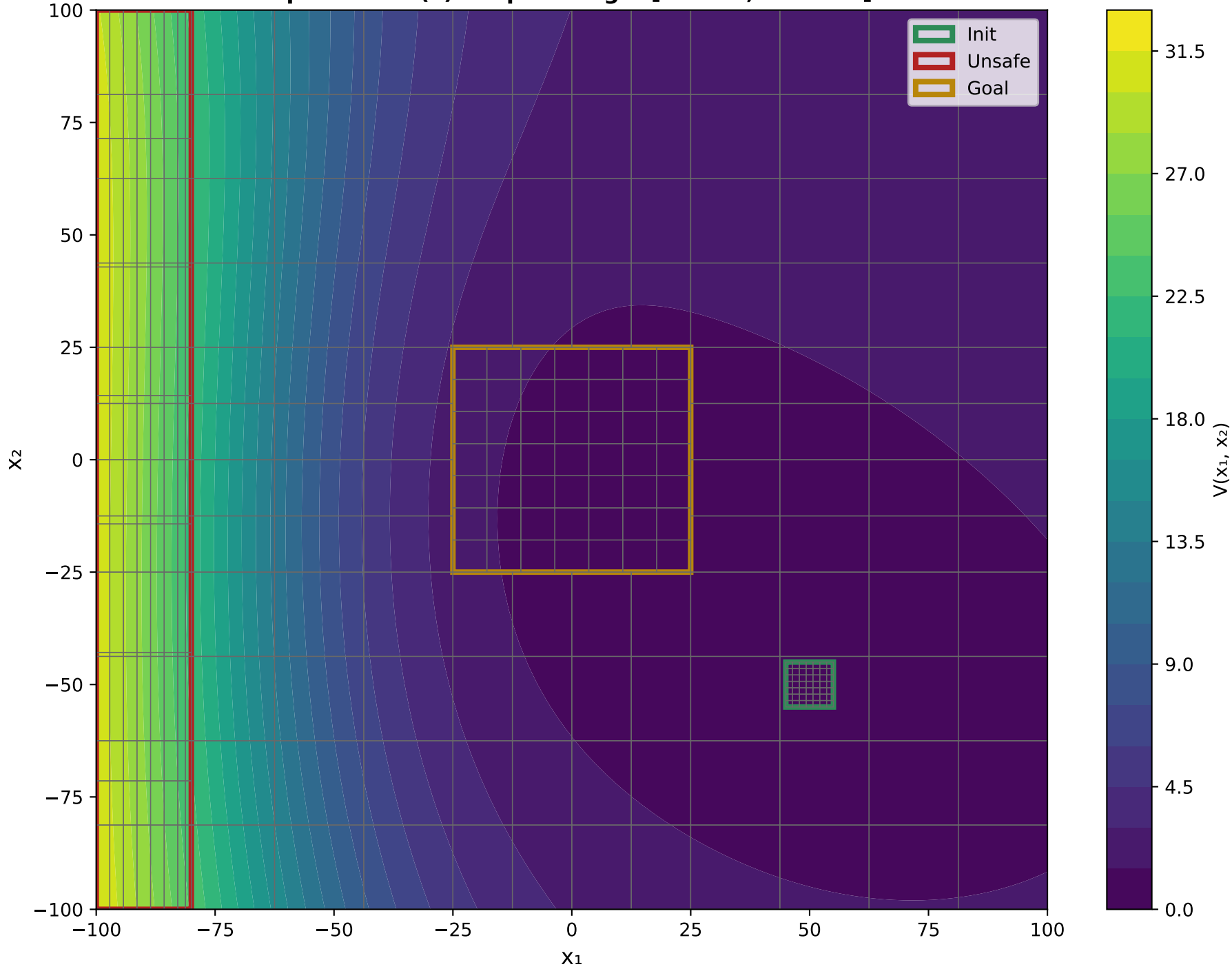
X 1 VS X 2 Epoch: 0 - V(x) Output Range: [0.7425, 31.6347]
