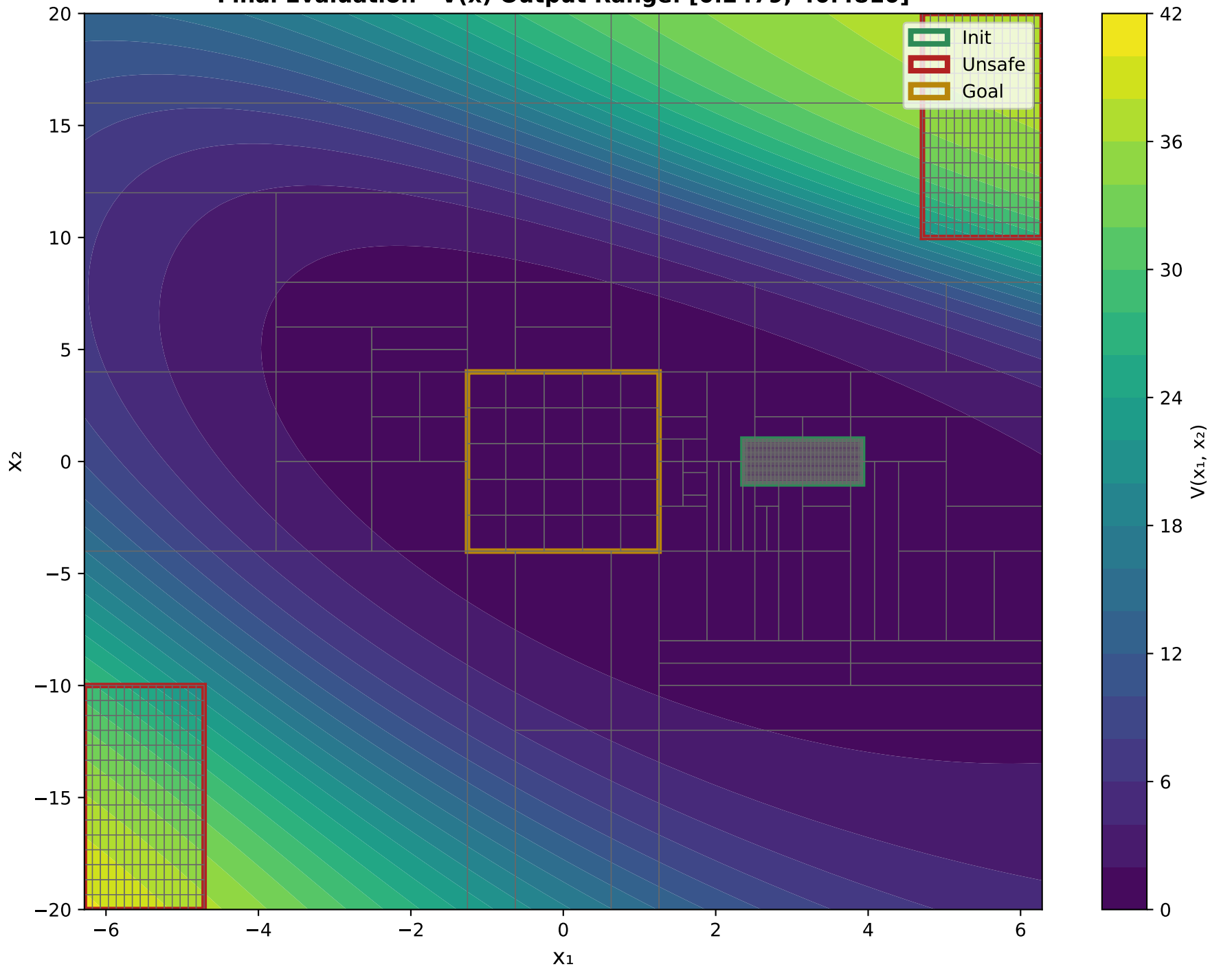
X 1 VS X 2 Final Evaluation - V(x) Output Range: [0.2479, 40.4810]
