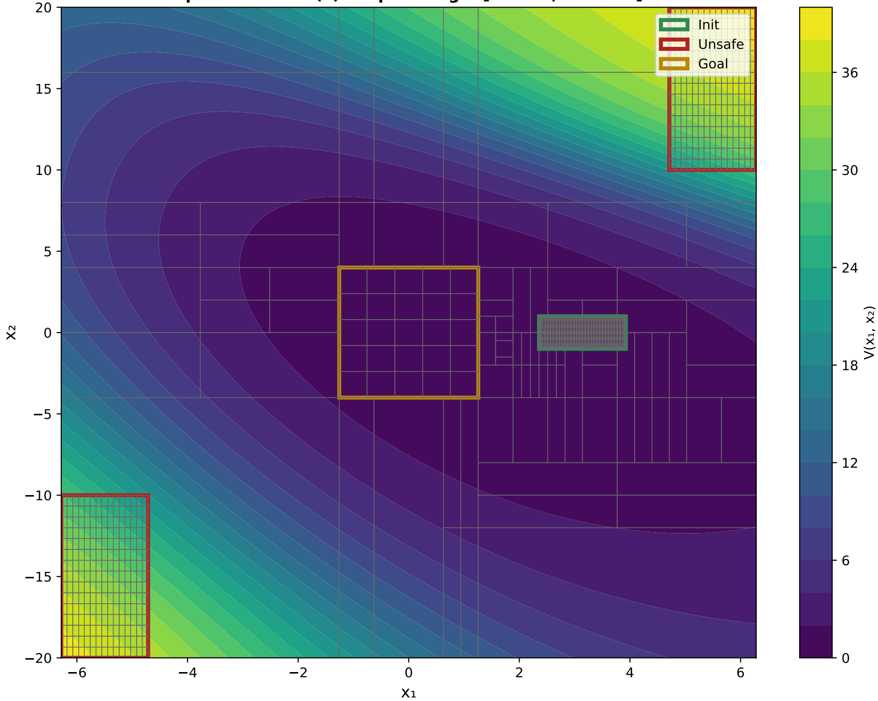
X 1 VS X 2 Epoch: 1000 - V(x) Output Range: [0.3538, 39.3093]
