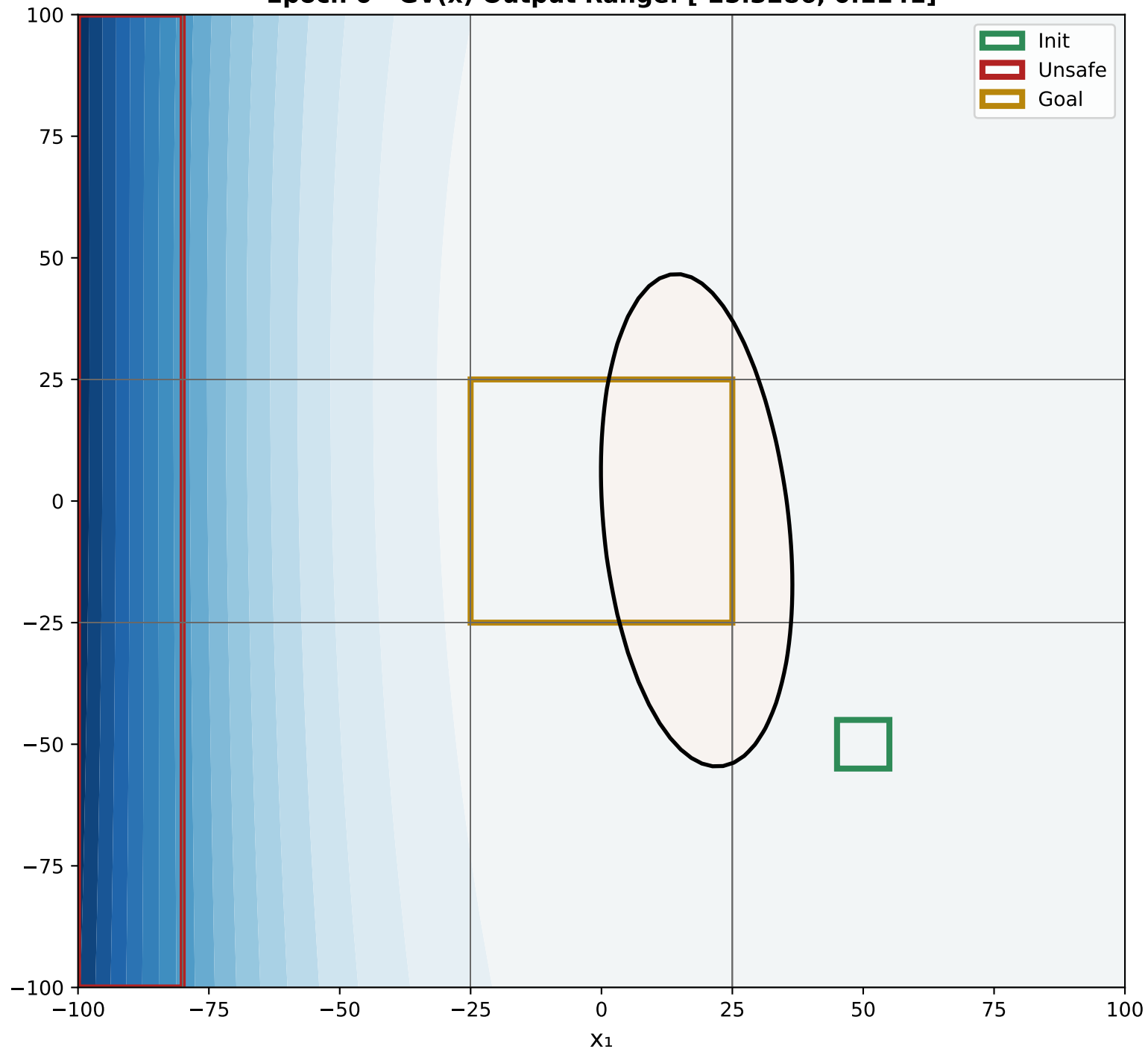
X 1 VS X 2 Epoch 0 - GV(x) Output Range: [-25.3286, 0.1141]
