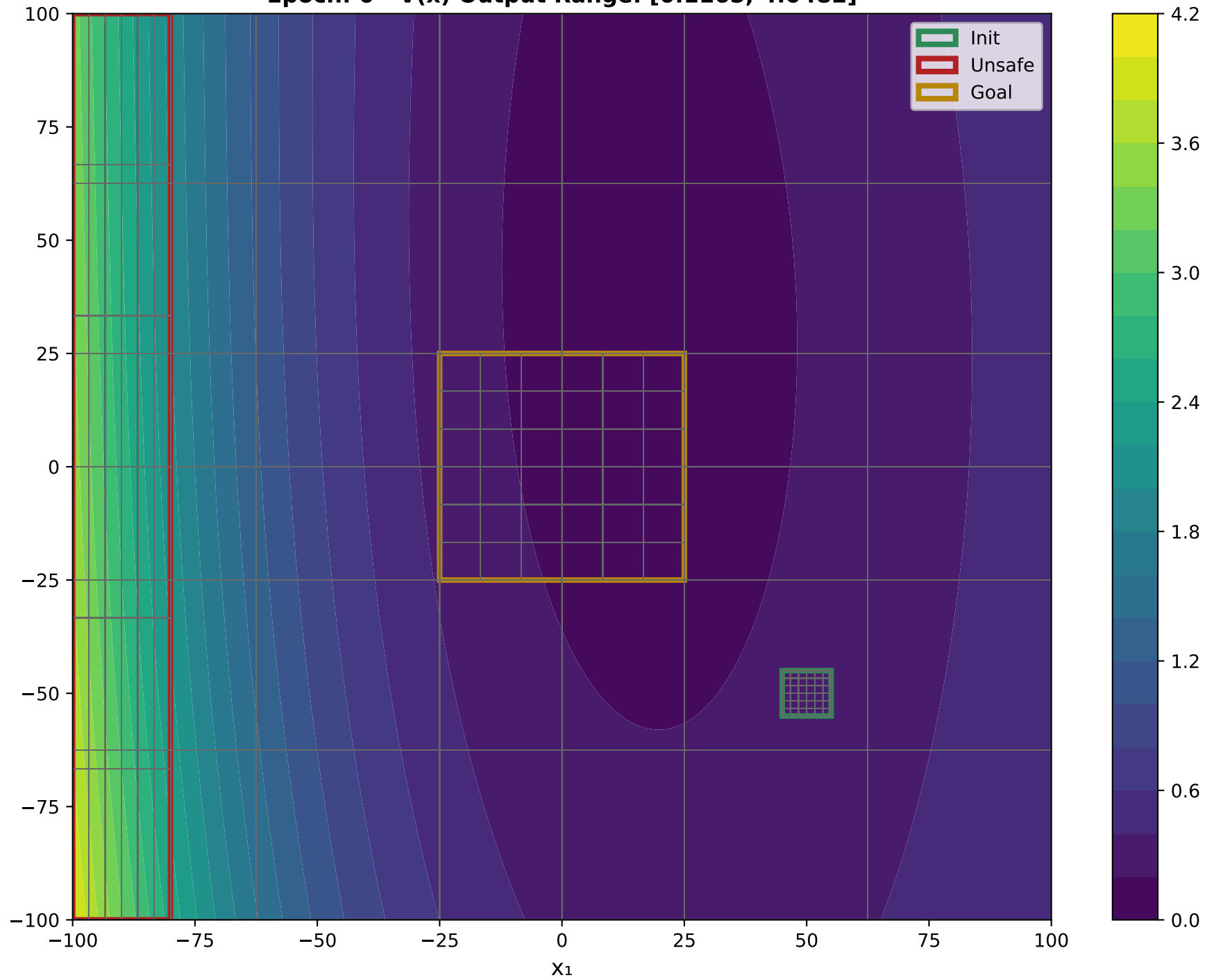
X 1 VS X 2 Epoch: 0 - V(x) Output Range: [0.1165, 4.0482]
