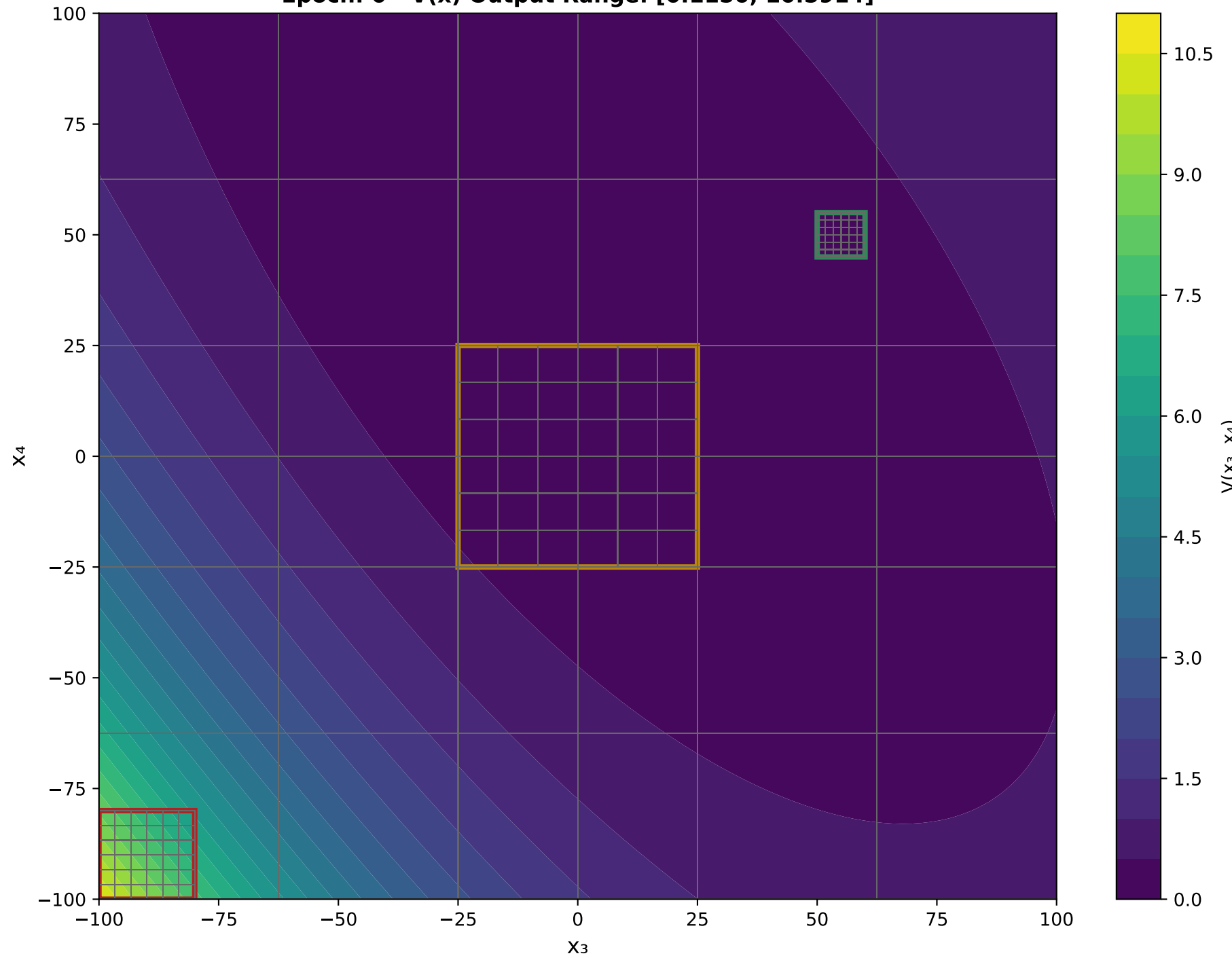
X 3 VS X 4 Epoch: 0 - V(x) Output Range: [0.1150, 10.5914]
