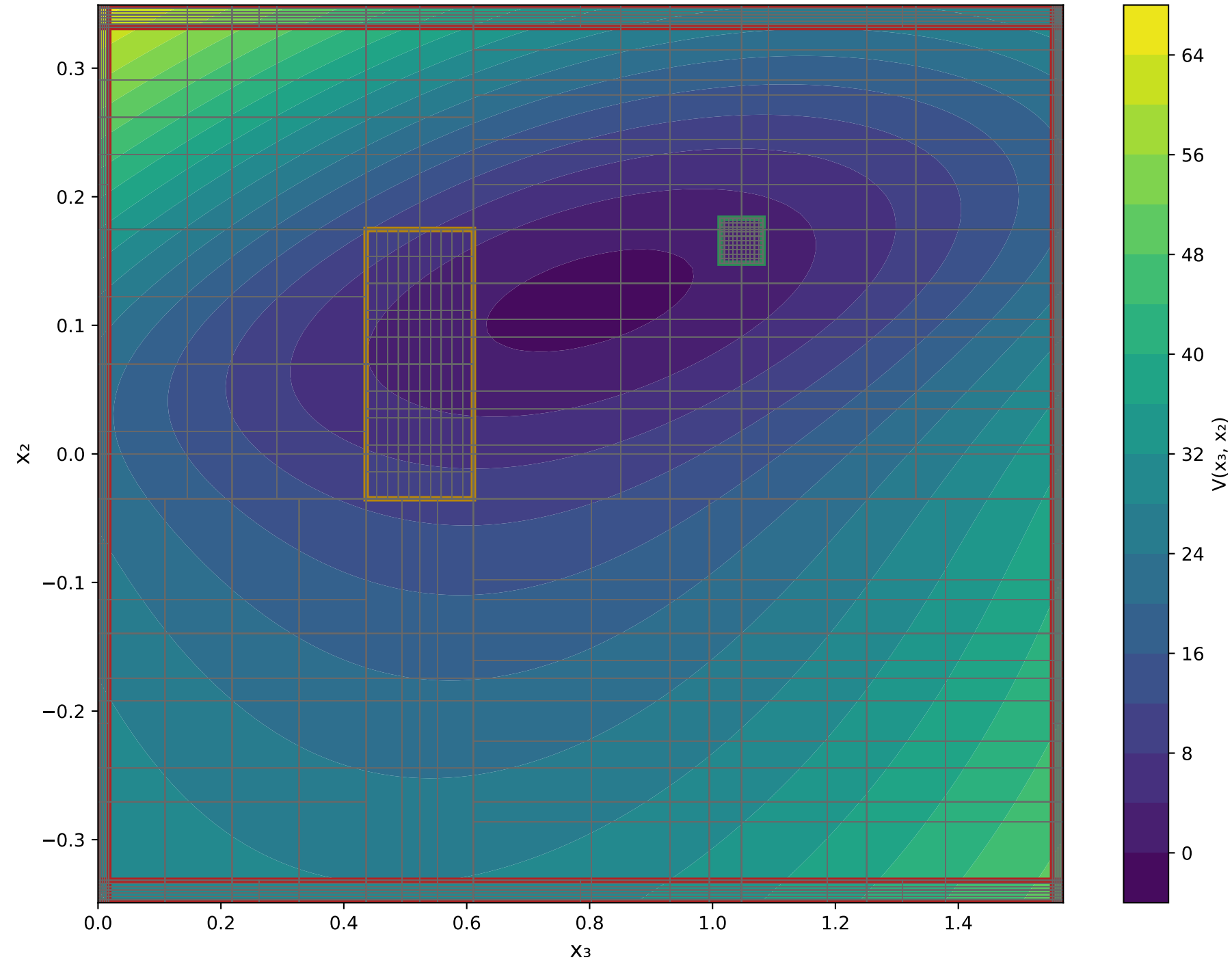
X 3 VS X 2 Epoch: 0 - V(x) Output Range: [-1.1160, 66.0490]
