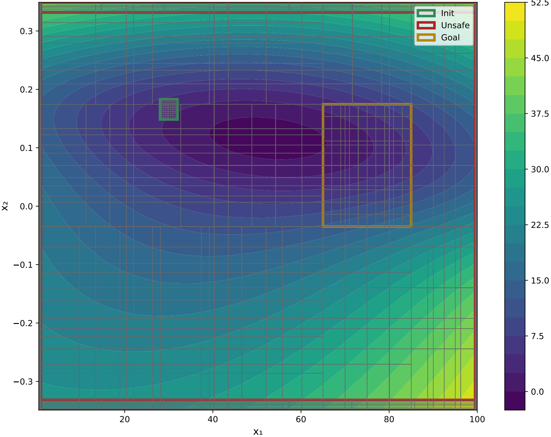
X 1 VS X 2 Epoch: 0 - V(x) Output Range: [-1.1478, 50.4865]
