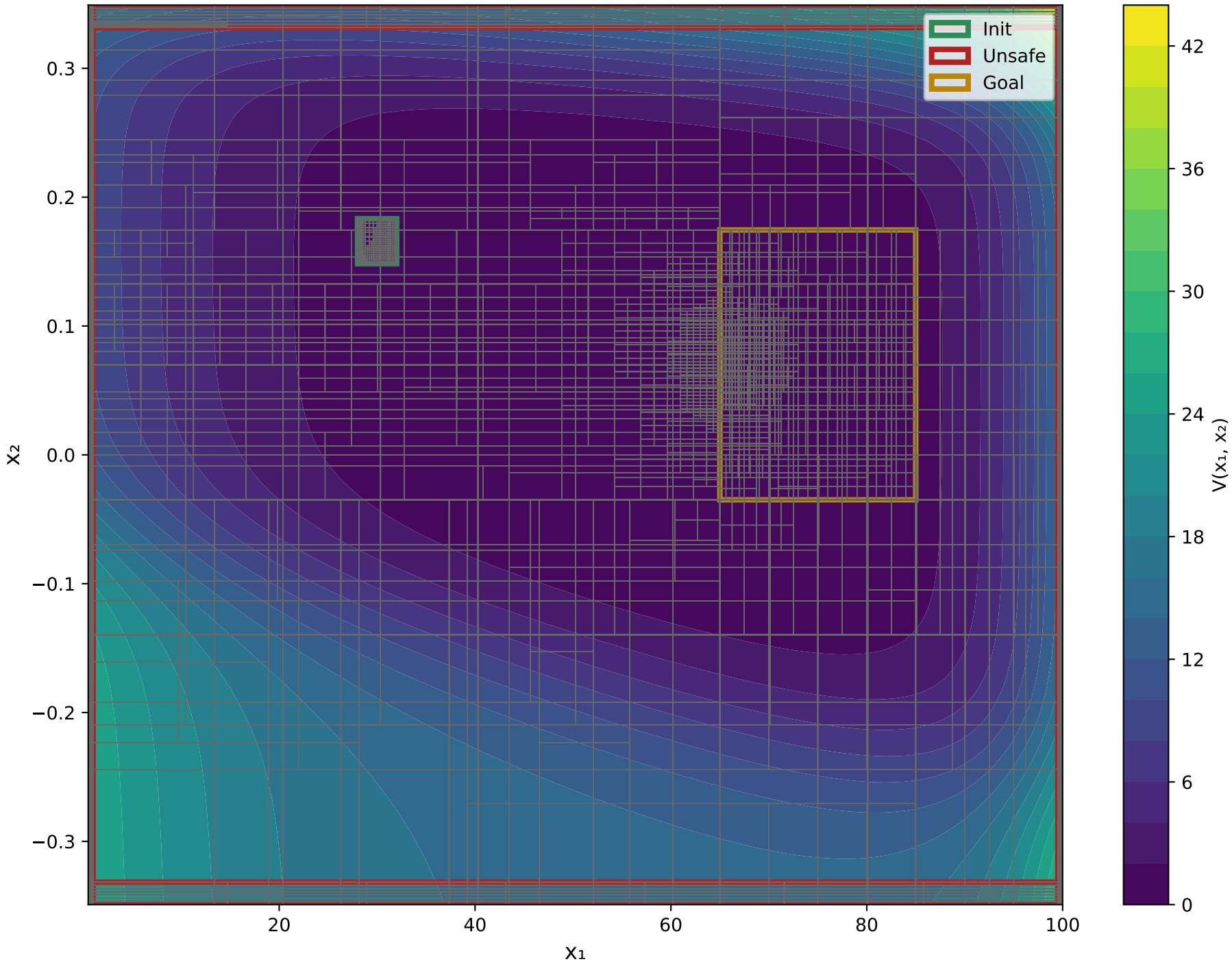
X 1 VS X 2 Epoch: 3000 - V(x) Output Range: [0.0440, 42.0423]
