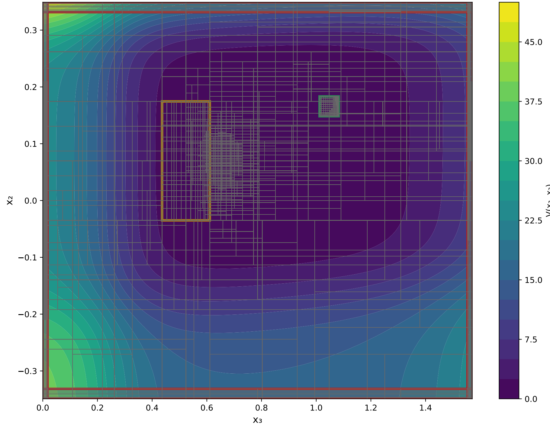
X 3 VS X 2 Epoch: 3000 - V(x) Output Range: [0.1022, 47.8744]
