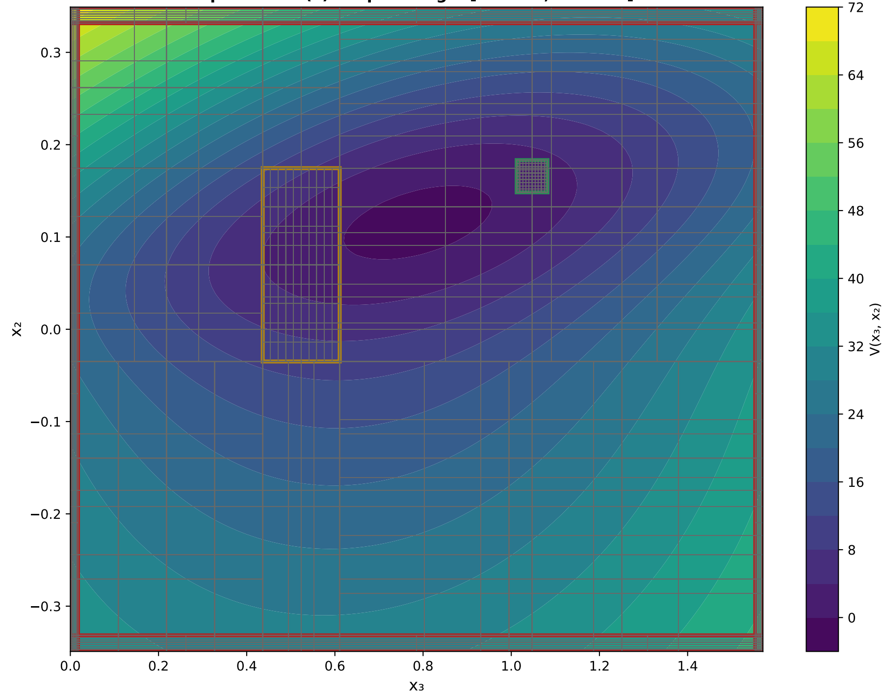
X 3 VS X 2 Epoch: 0 - V(x) Output Range: [-1.1693, 70.9829]
