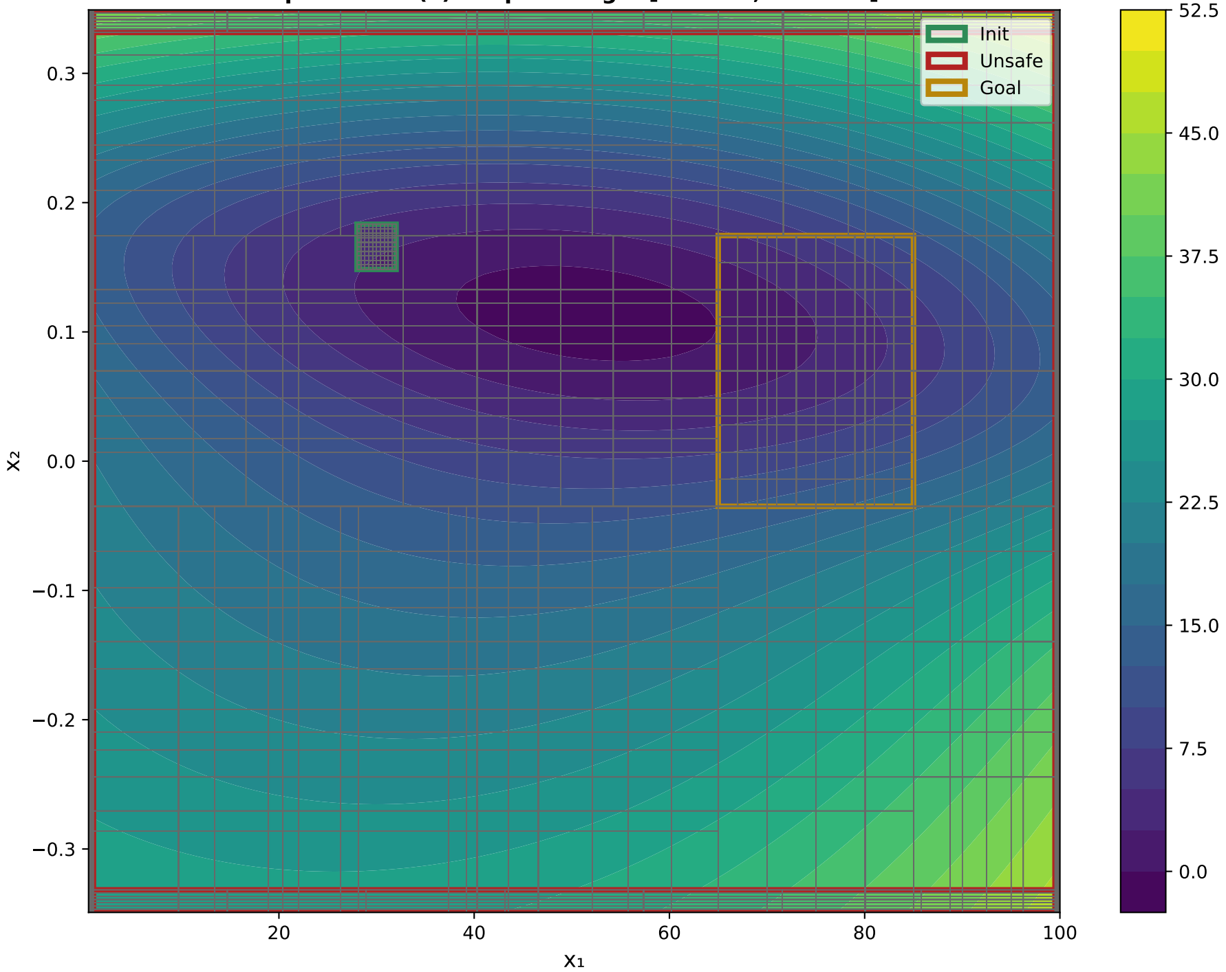
X 1 VS X 2 Epoch: 0 - V(x) Output Range: [-1.1769, 50.7064]
