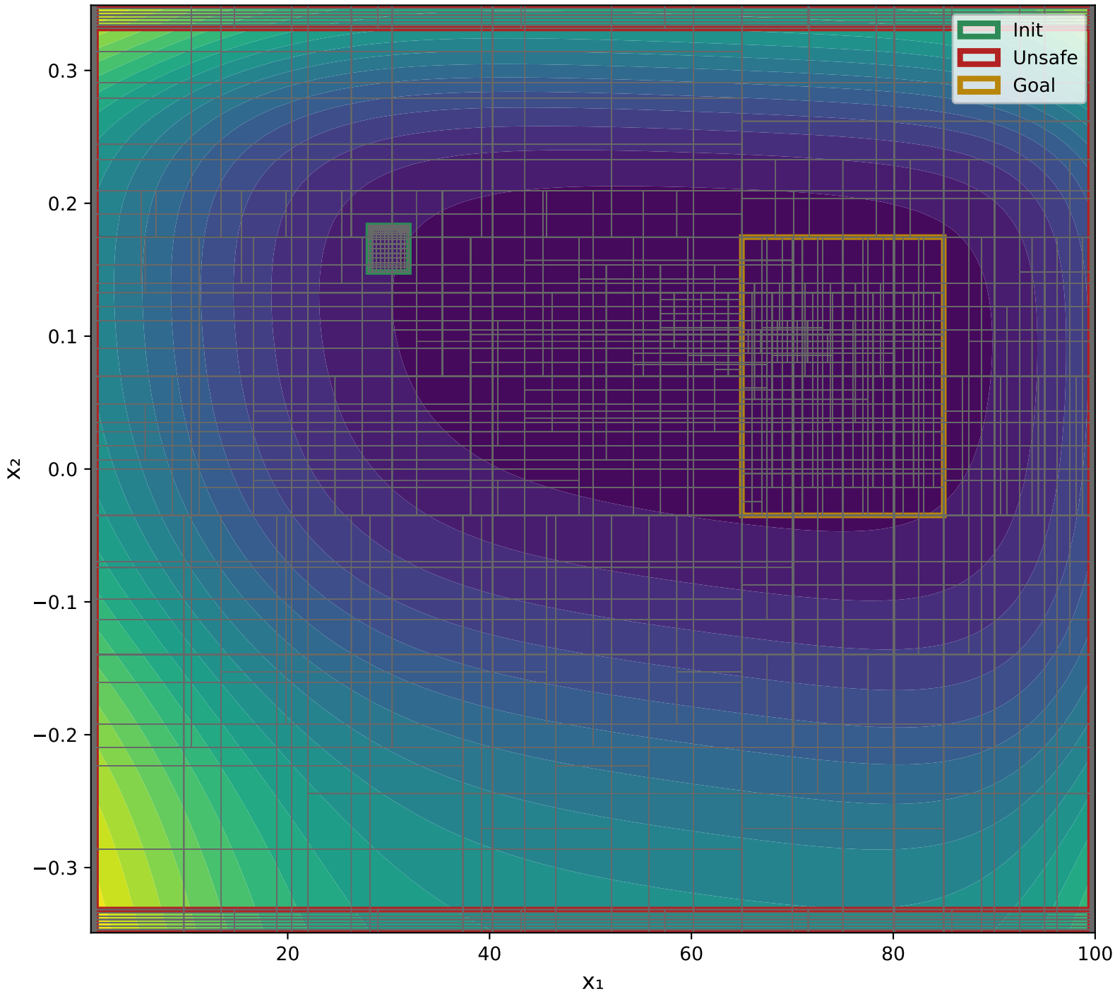
X 1 VS X 2 Epoch: 2000 - V(x) Output Range: [0.0371, 37.4910]
