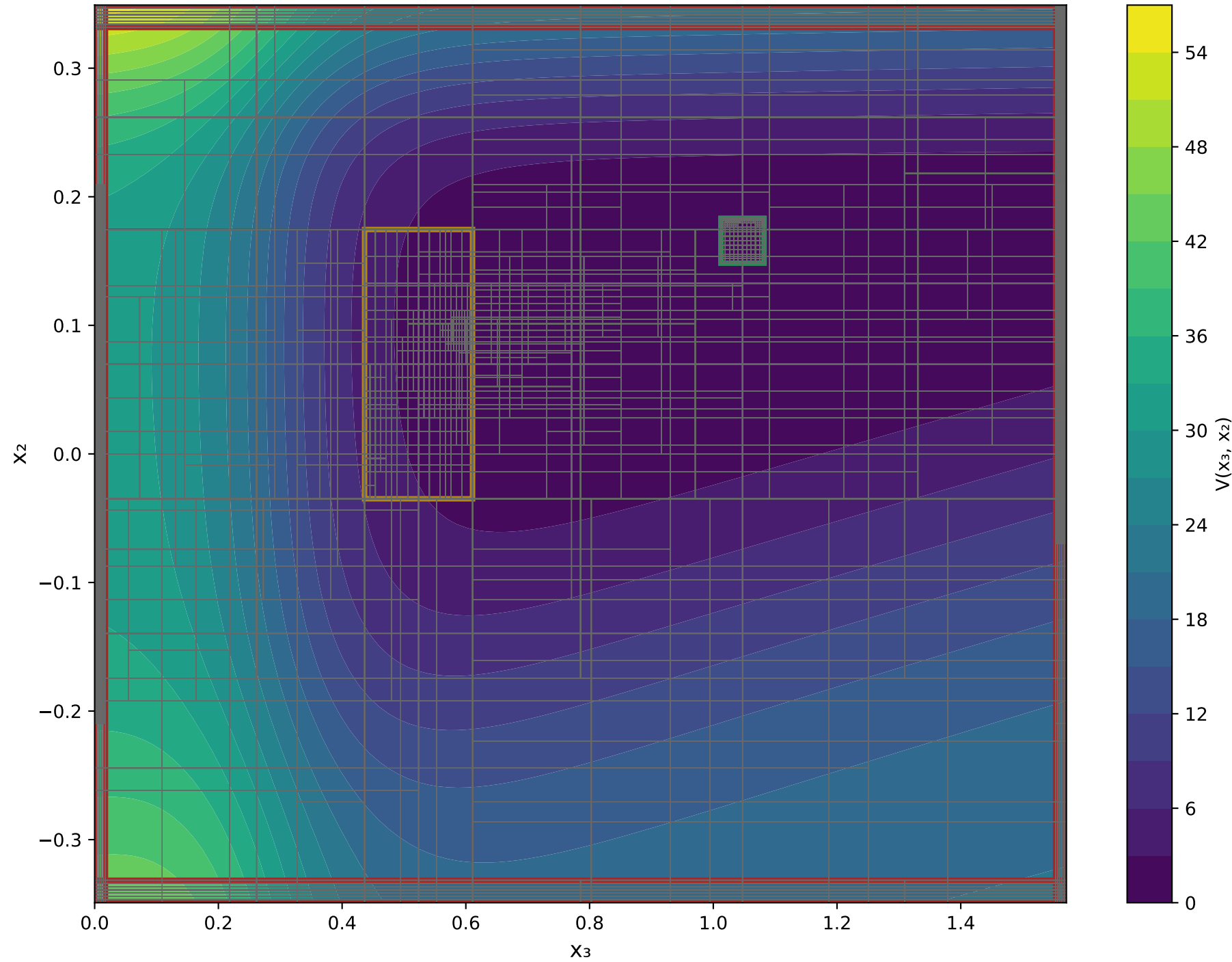
X 3 VS X 2 Epoch: 2000 - V(x) Output Range: [0.1797, 55.4675]
