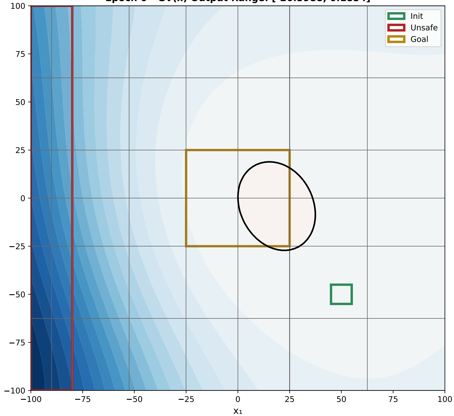
X 1 VS X 2 Epoch 0 - GV(x) Output Range: [-26.5988, 0.1854]
