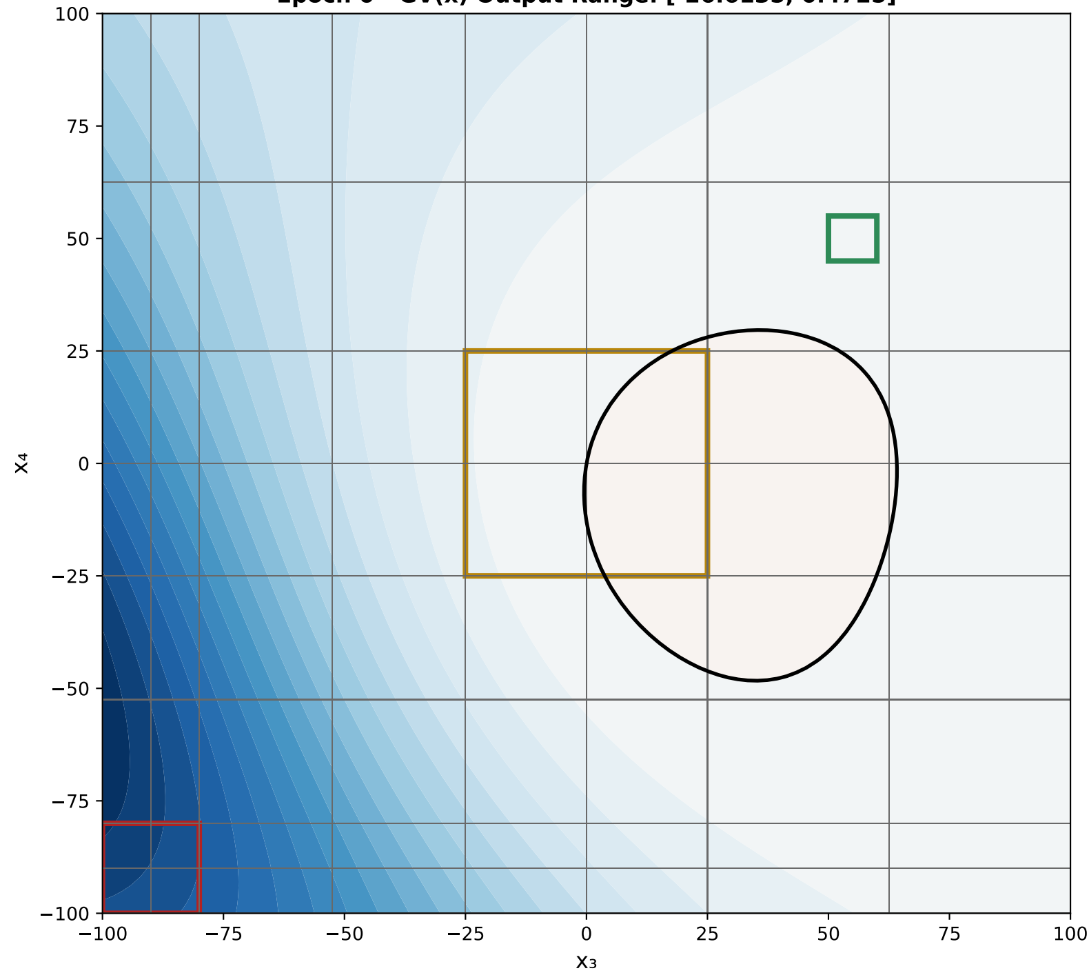
X 3 VS X 4 Epoch 0 - GV(x) Output Range: [-26.6135, 0.4725]
