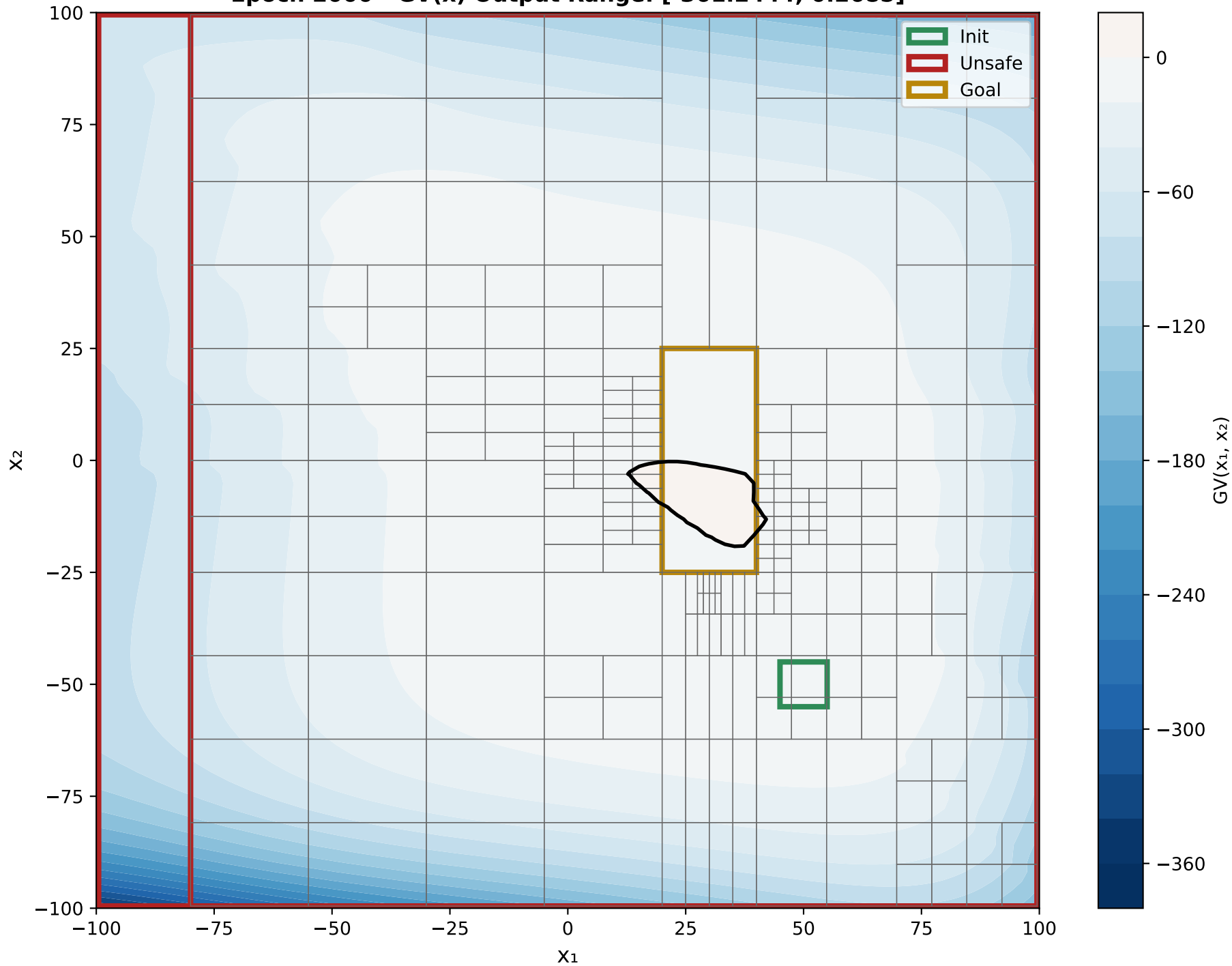
X 1 VS X 2 Epoch 2000 - GV(x) Output Range: [-361.2444, 0.2685]
