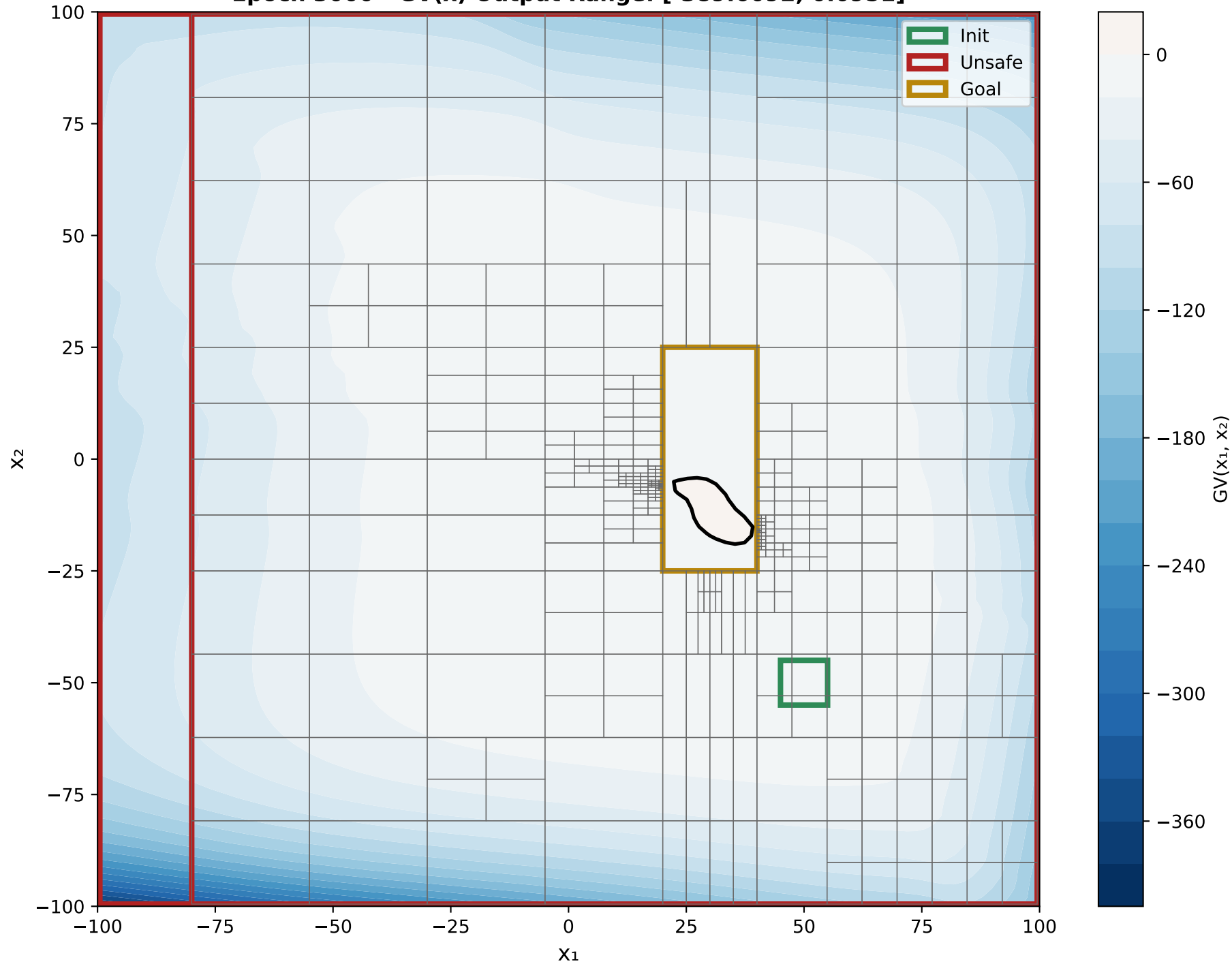
X 1 VS X 2 Epoch 3000 - GV(x) Output Range: [-389.6092, 0.0951]
