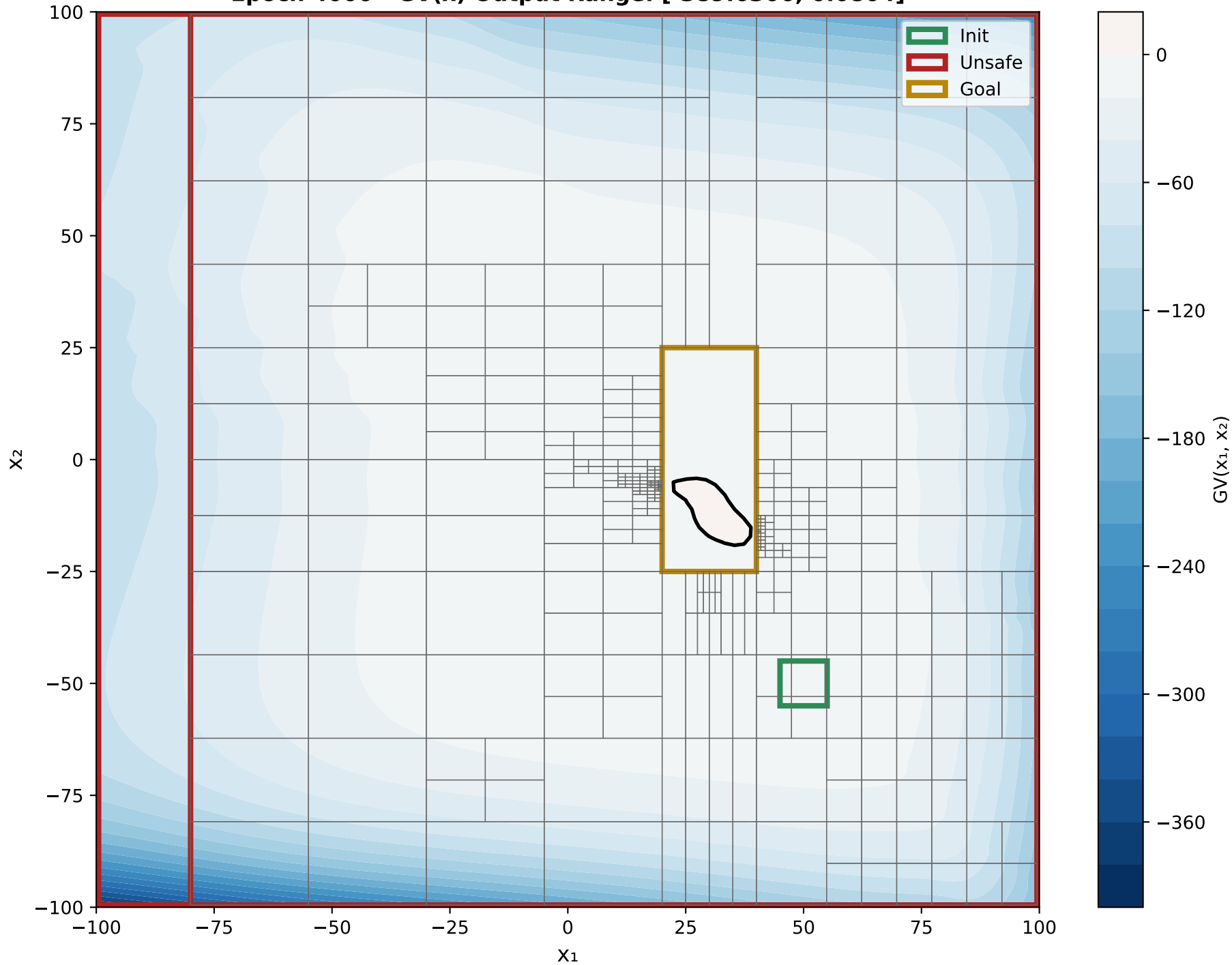
X 1 VS X 2 Epoch 4000 - GV(x) Output Range: [-389.6306, 0.0804]
