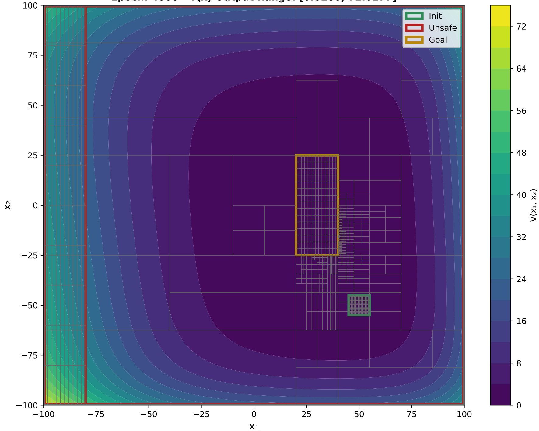
X 1 VS X 2 Epoch: 4000 - V(x) Output Range: [0.0280, 72.0277]
