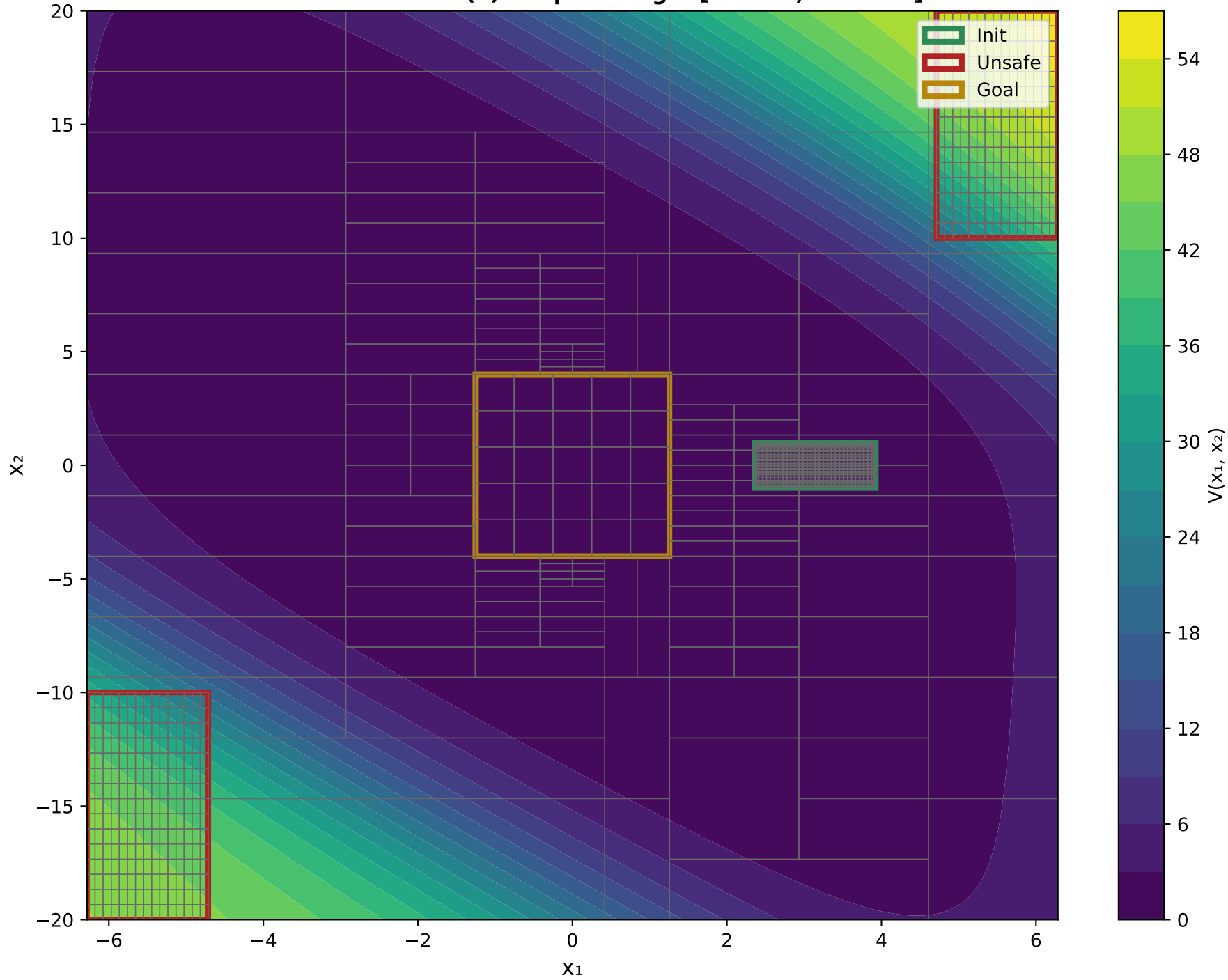
X 1 VS X 2 Final Evaluation - V(x) Output Range: [0.0544, 55.3397]
