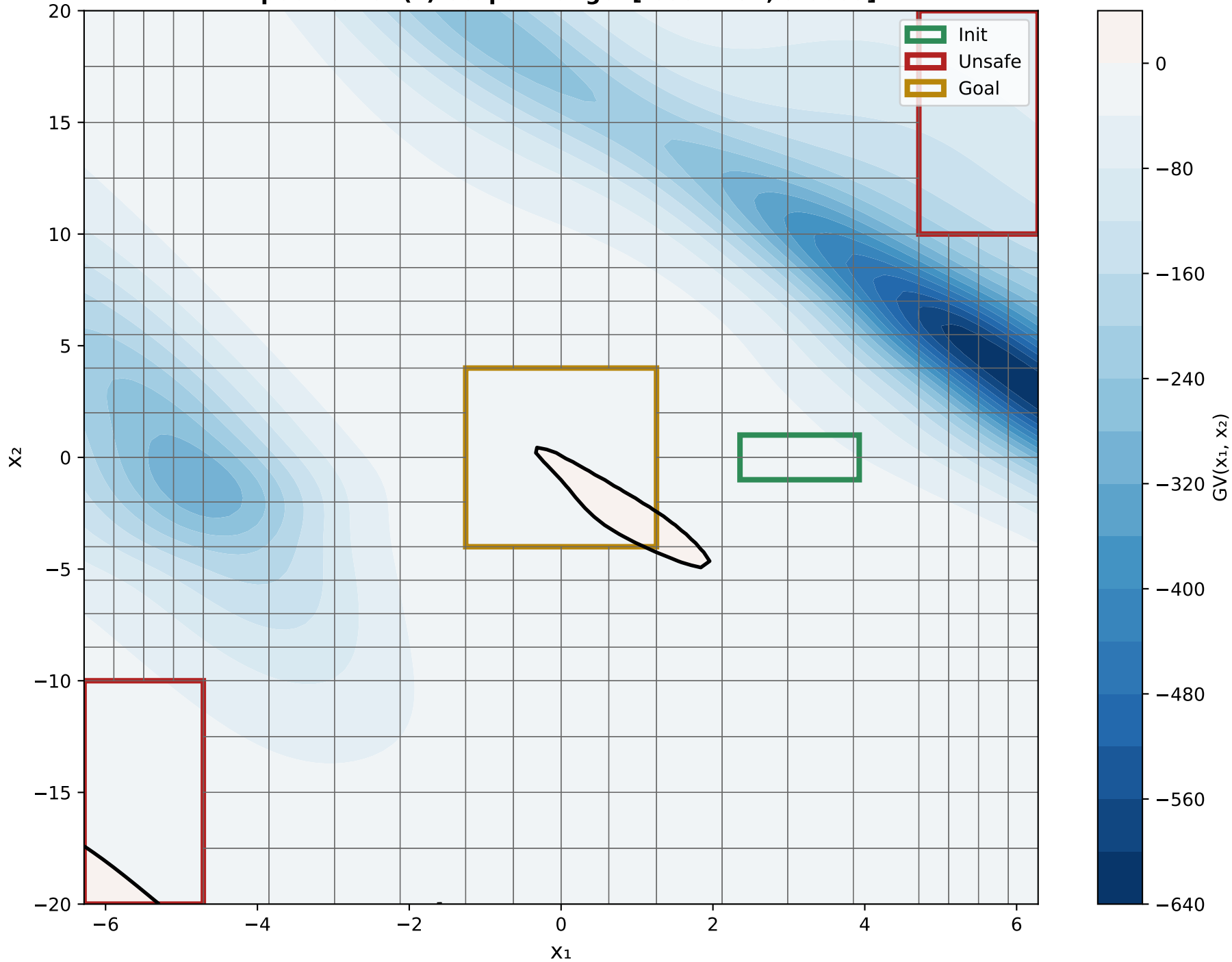
X 1 VS X 2 Epoch 0 - GV(x) Output Range: [-639.1294, 3.6609]
