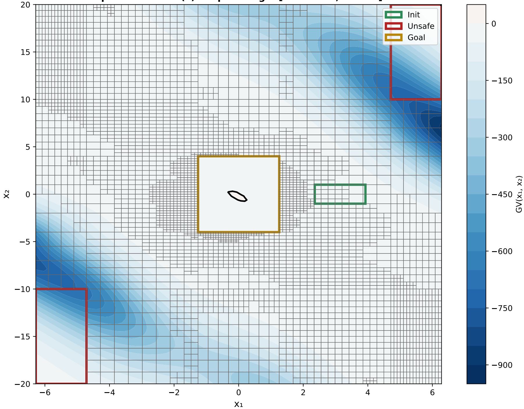
X 1 VS X 2 Epoch 1000 - GV(x) Output Range: [-910.9372, 1.3343]
