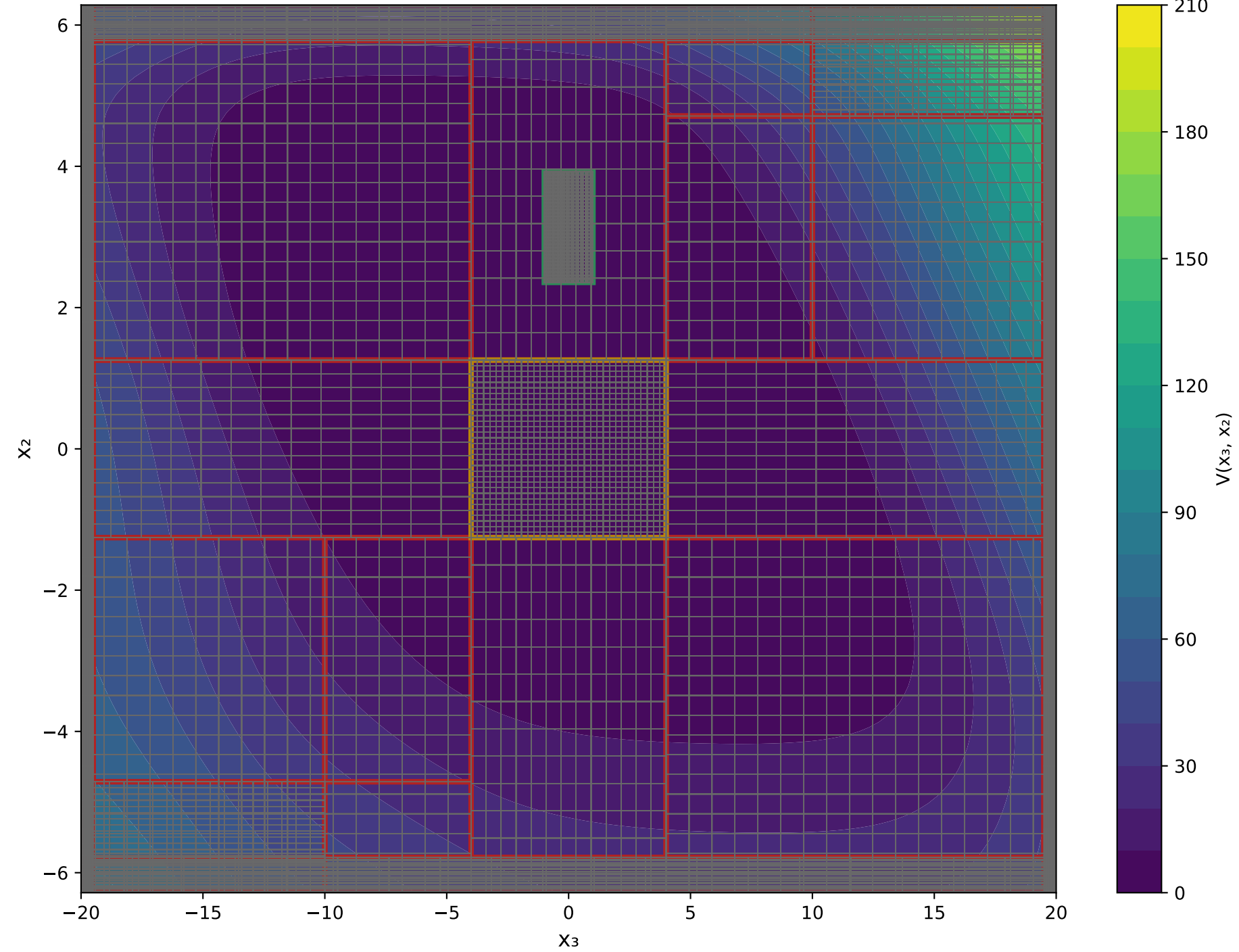
X 3 VS X 2 Epoch: 0 - V(x) Output Range: [0.0400, 200.3701]
