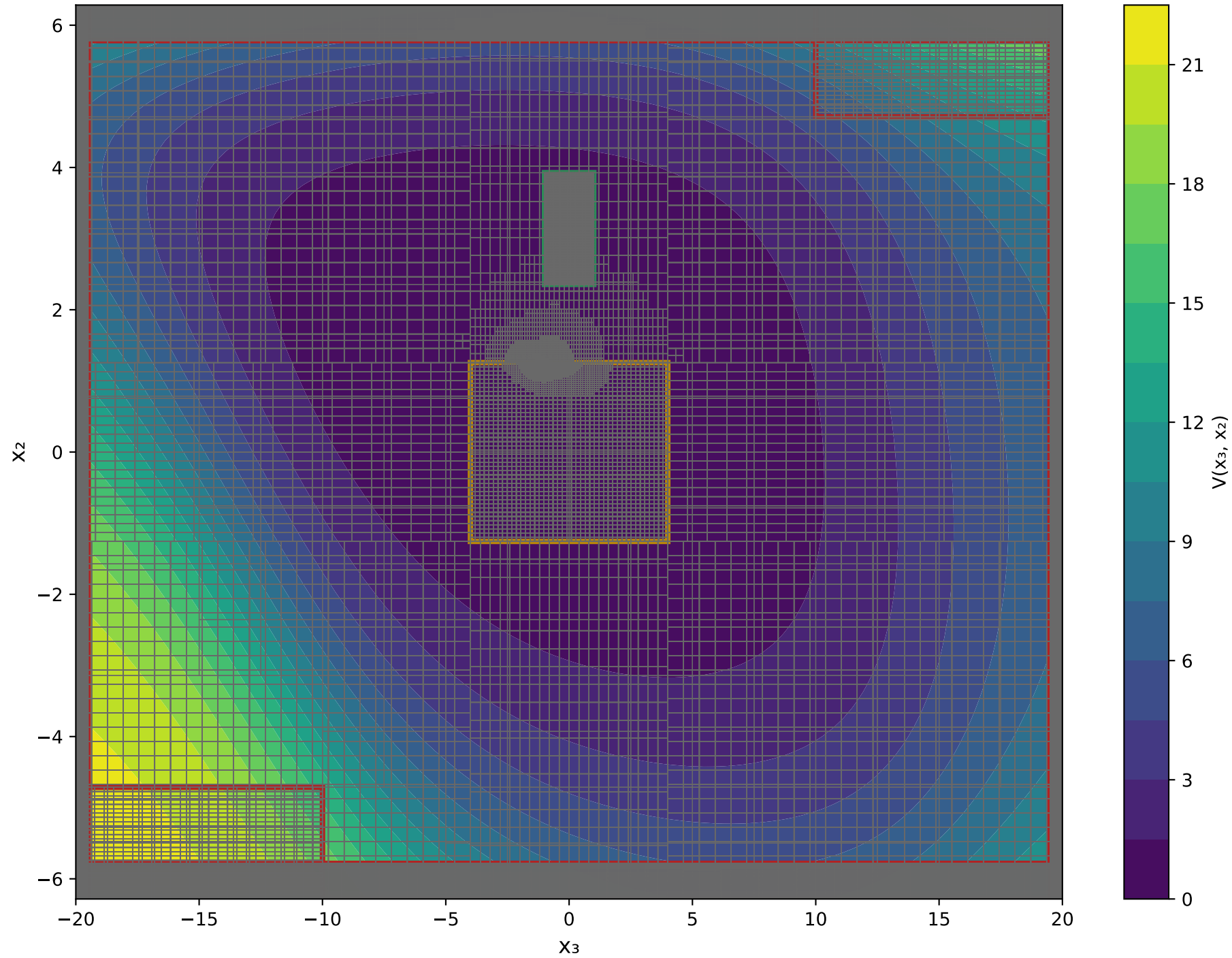
X 3 VS X 2 Epoch: 2000 - V(x) Output Range: [0.0741, 22.1326]
