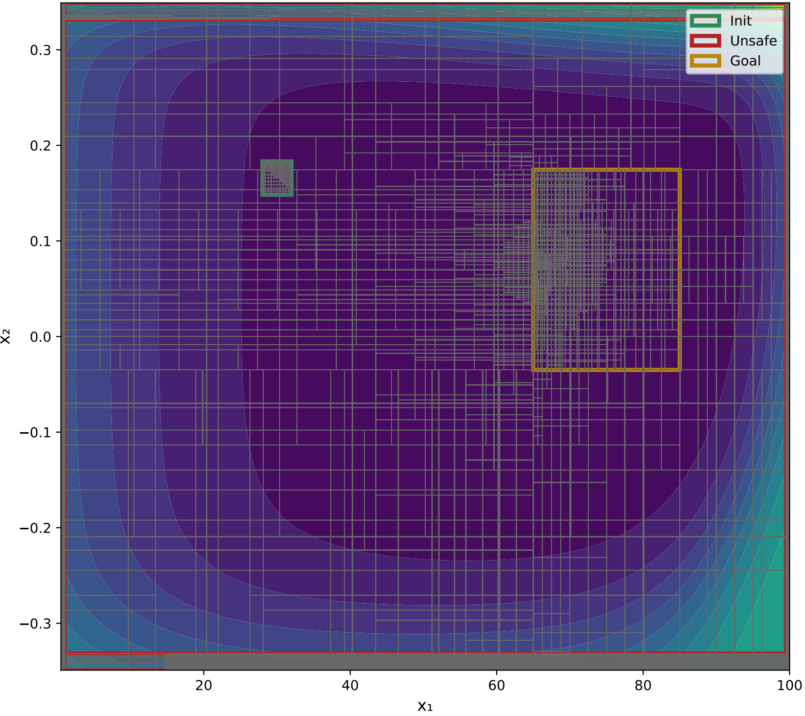
X 1 VS X 2 Epoch: 6000 - V(x) Output Range: [2.3043, 34.1710]
