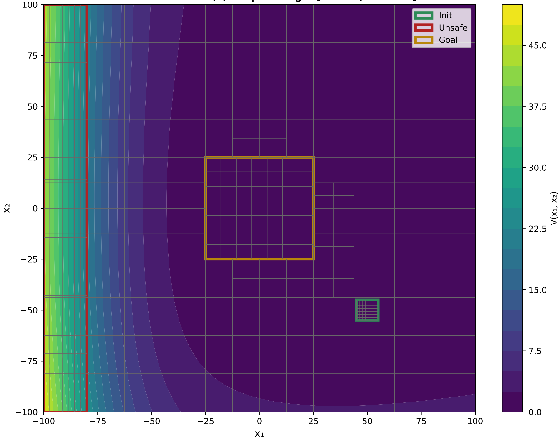
X 1 VS X 2 Final Evaluation - V(x) Output Range: [0.1810, 48.0768]
