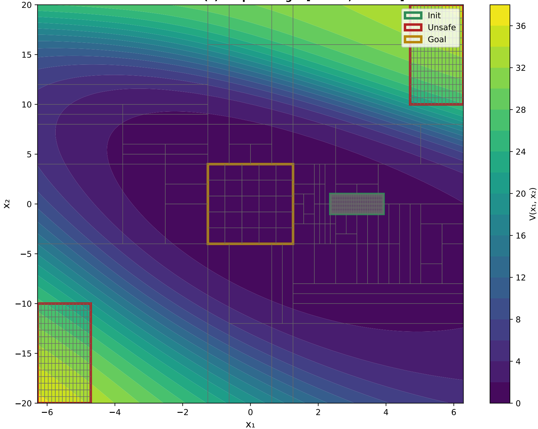
X 1 VS X 2 Final Evaluation - V(x) Output Range: [0.2333, 36.6234]
