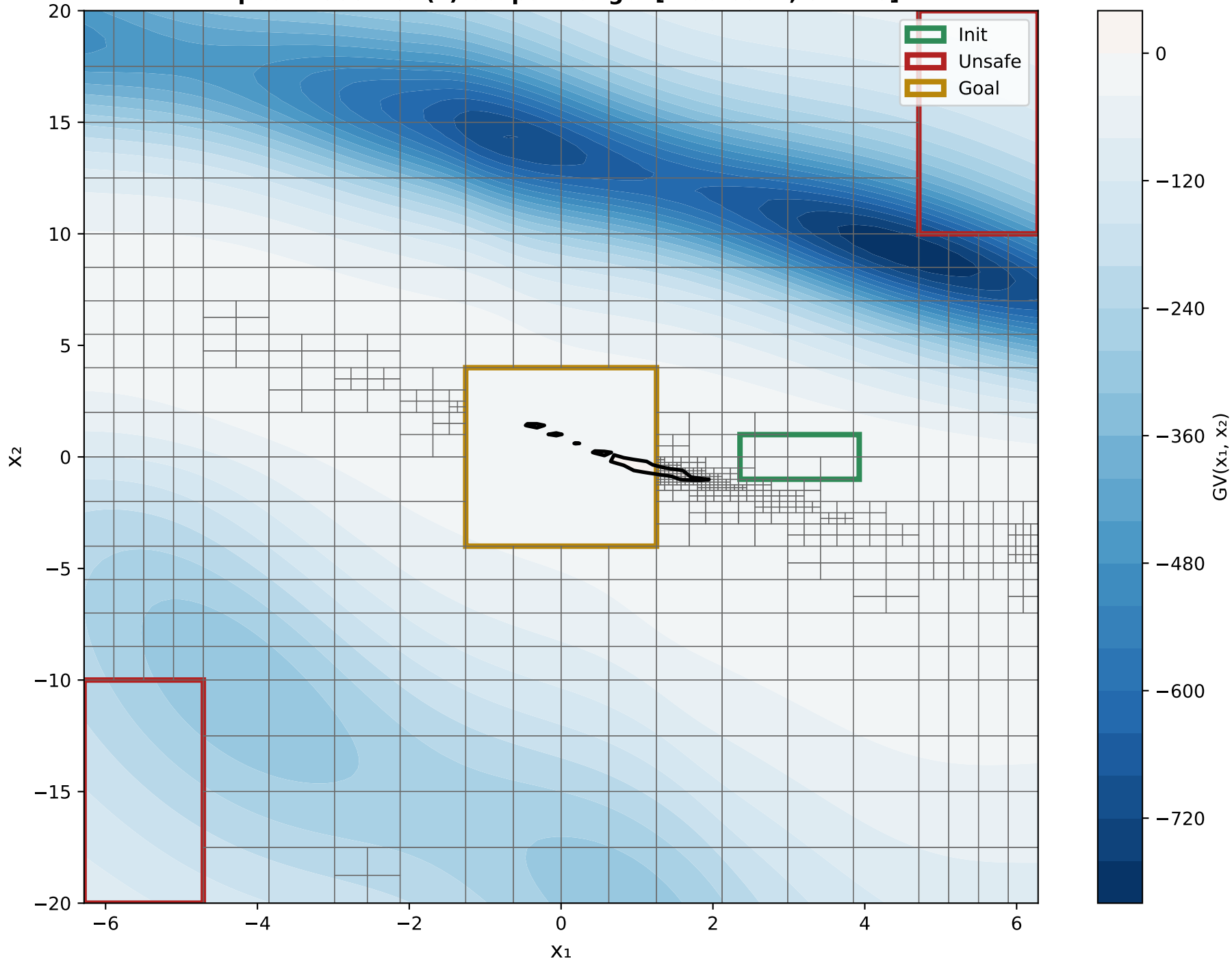
X 1 VS X 2 Epoch 1000 - GV(x) Output Range: [-796.0312, 0.1240]
