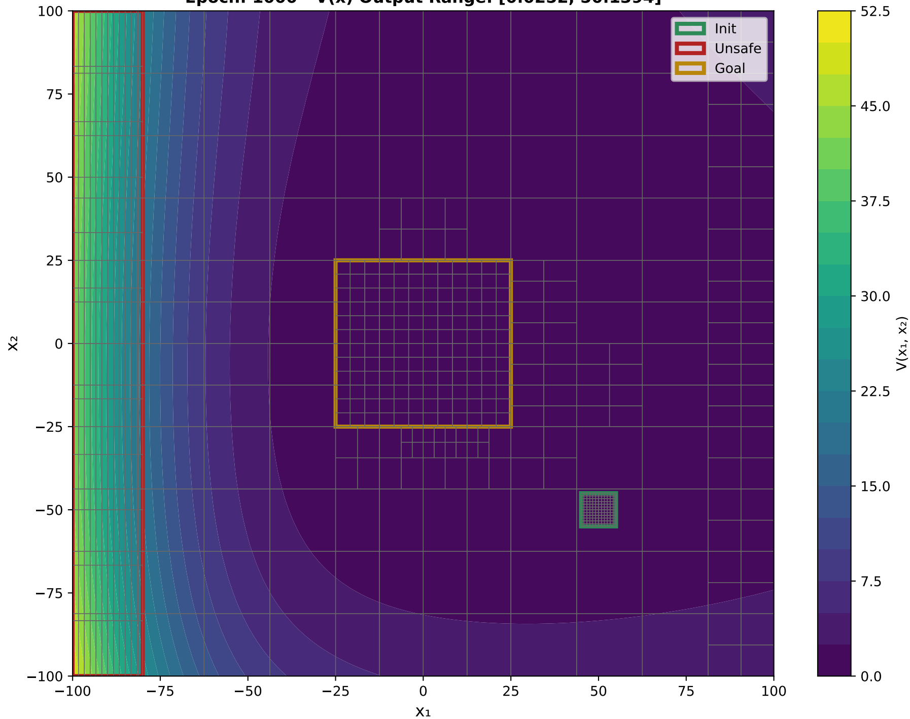
X 1 VS X 2 Epoch: 1000 - V(x) Output Range: [0.0252, 50.1394]
