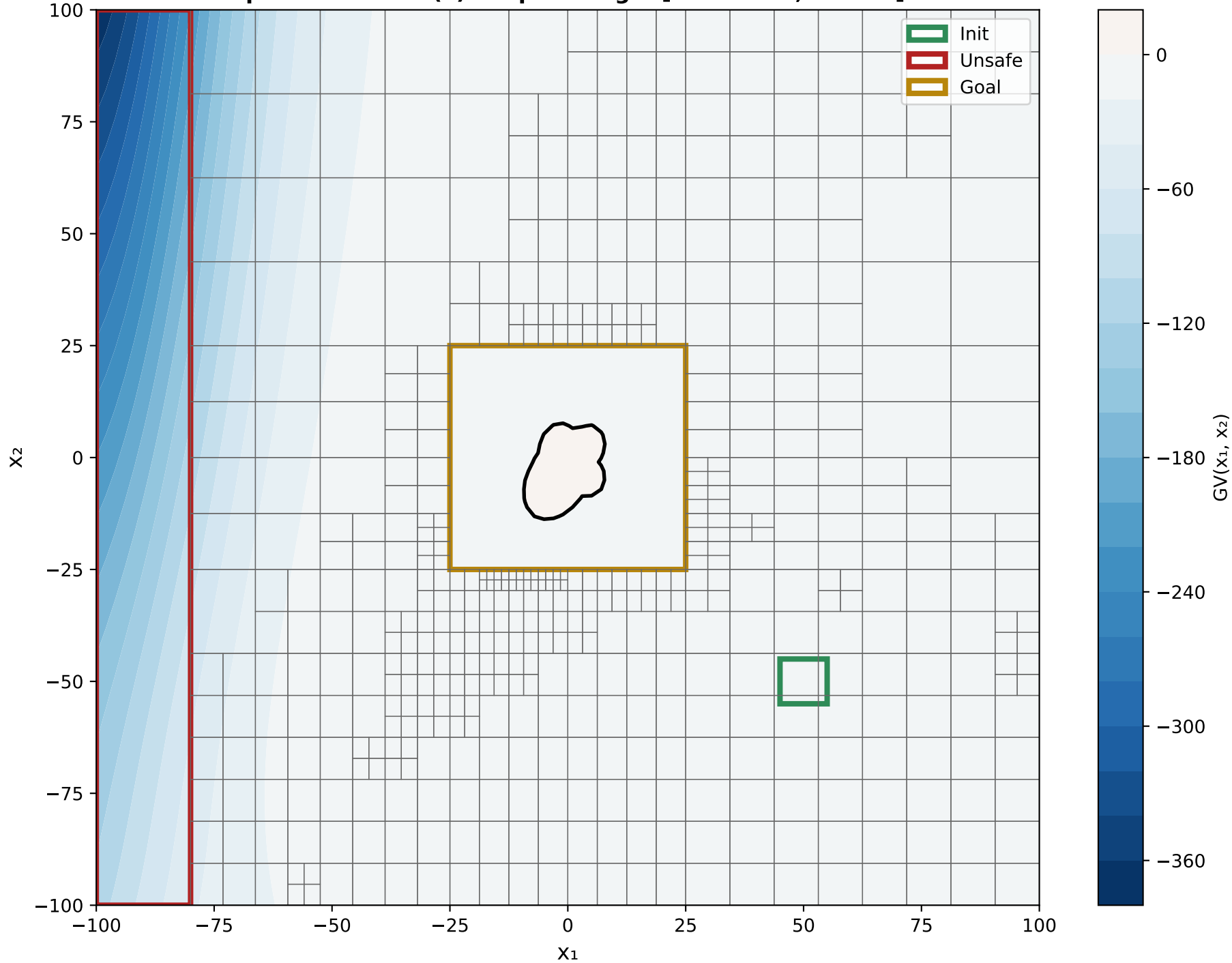
X 1 VS X 2 Epoch 1000 - GV(x) Output Range: [-376.5366, 0.0371]
